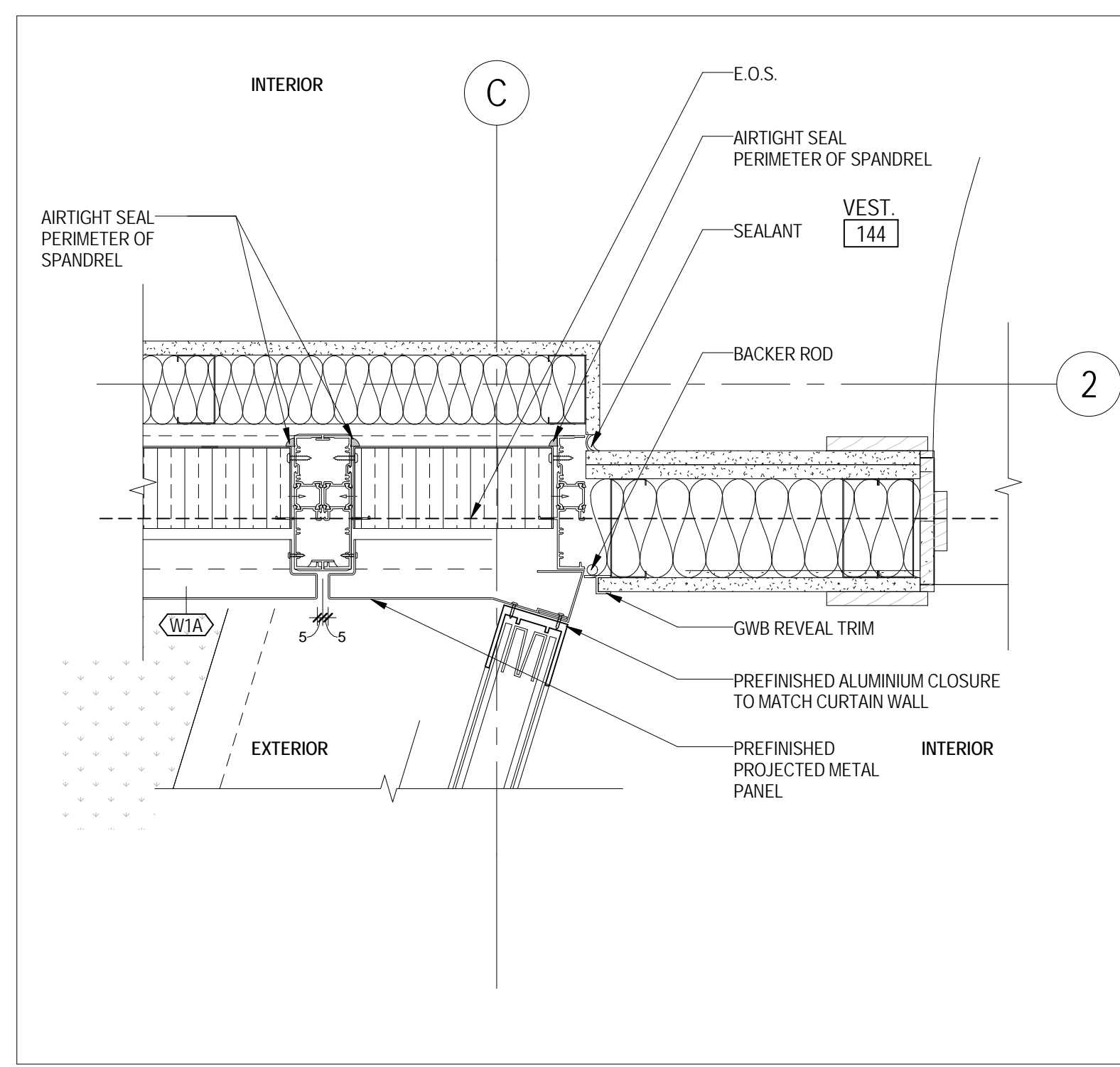
3 A 240 GL4 ALTERNATE PLAN DETAIL AT AMENITY / FITNESS 1:5
