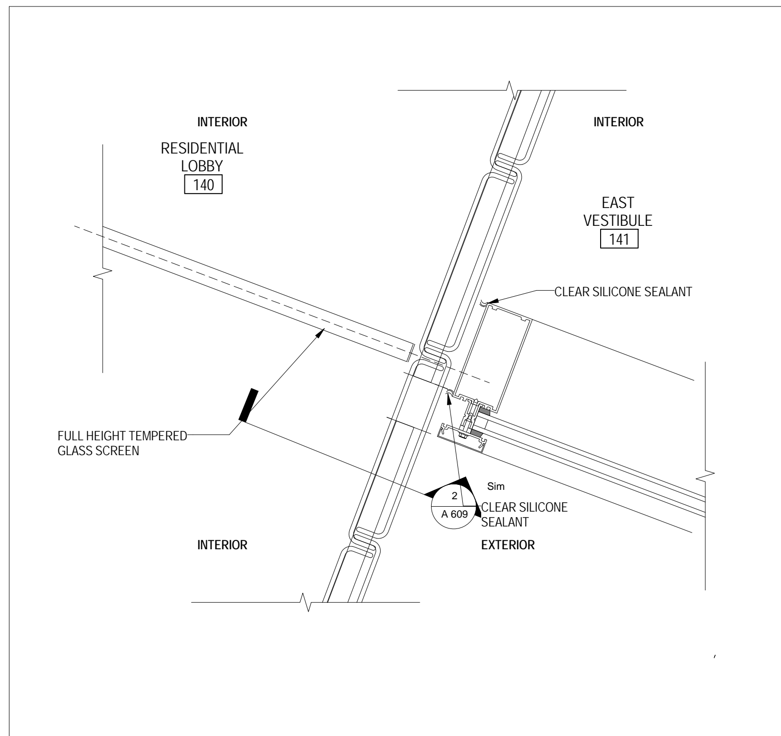
4 A 240 GL4 ALTERNATE PLAN DETAIL AT EAST VESTIBULE 1:5
