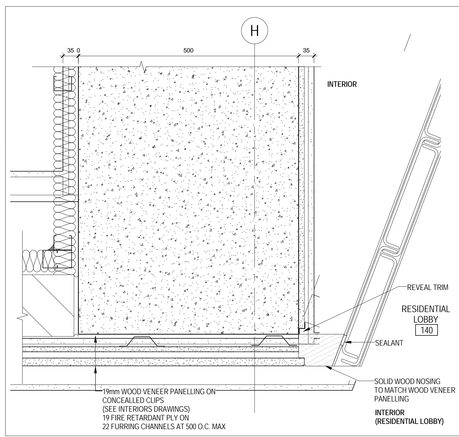
5 A 240 GL4 ALTERNATE PLAN DETAIL AT GRID H / 10 1:5
