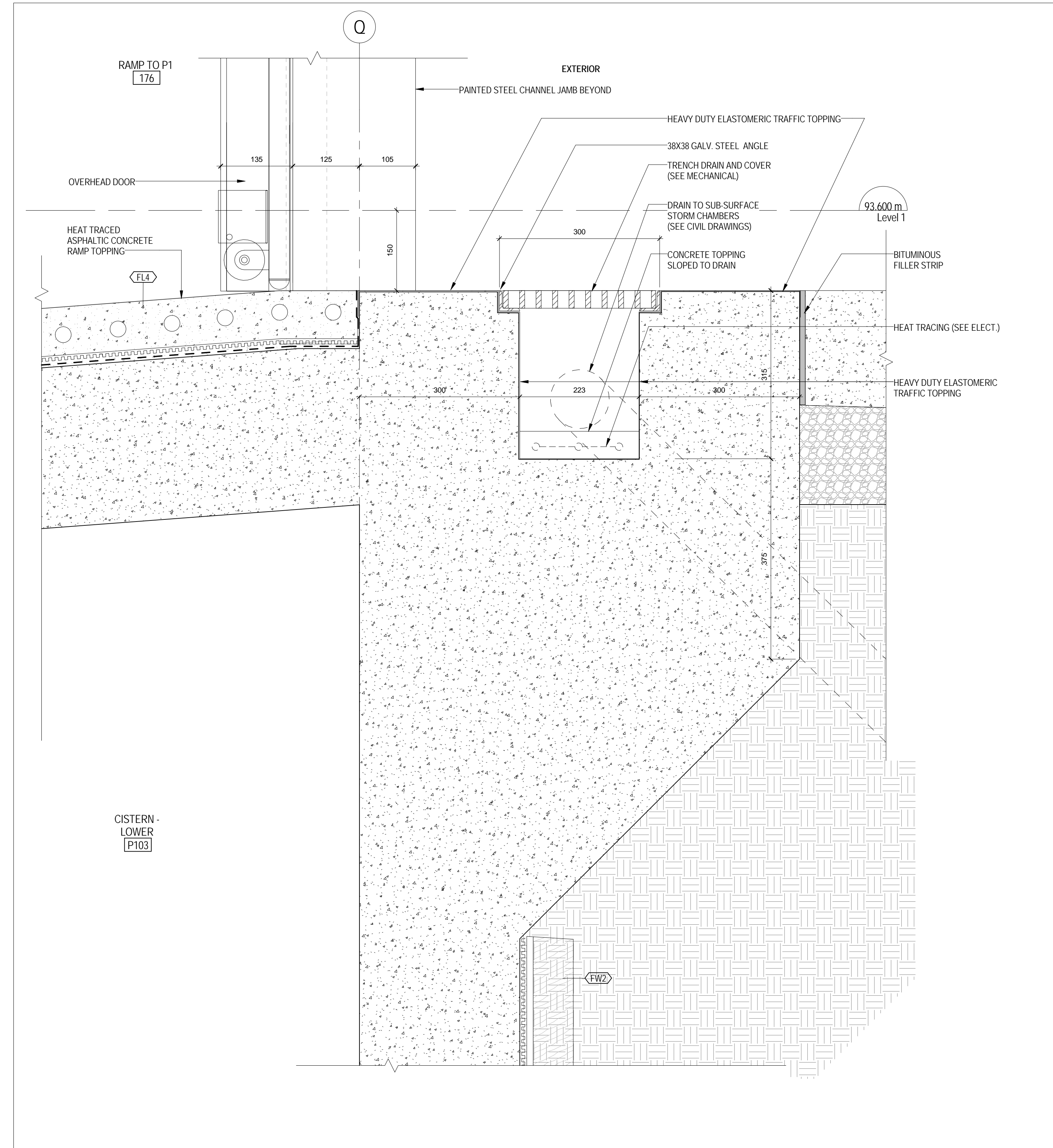
1 A 610 1:5 FOUNDATION WALL AT RAMP TO P1
