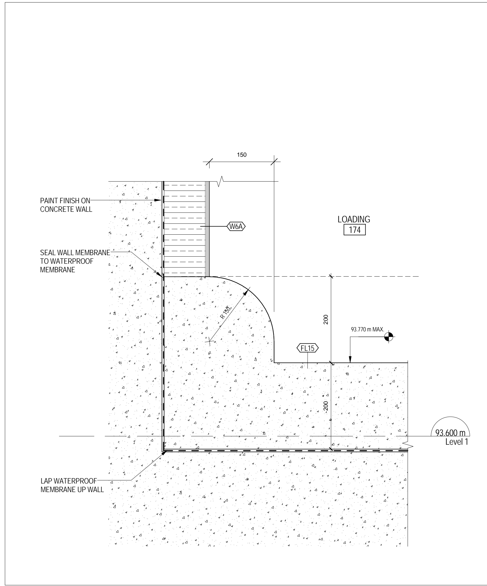
5 A 610 1:5 LOADING DOCK CURB EAST WALL
