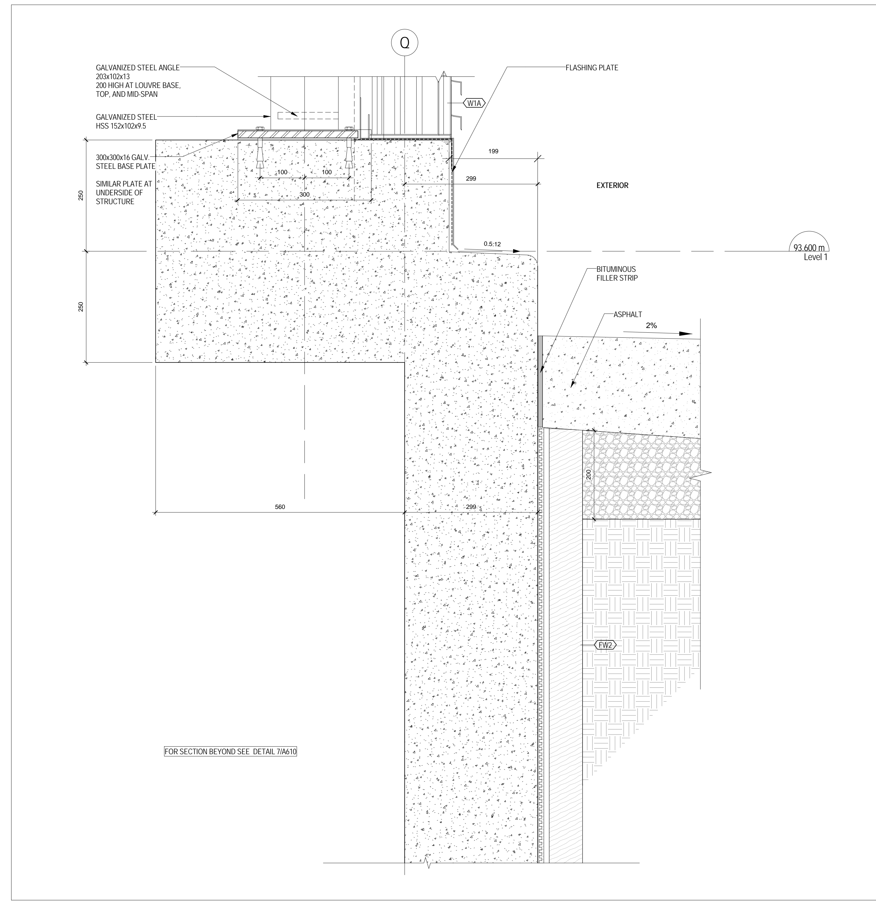
2 A 610 1:5 FOUNDATION WALL AT LOUVER BASE
