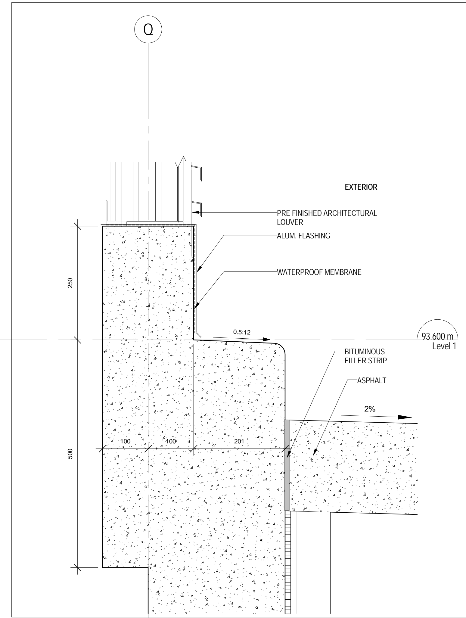
7 A 610 1:5 LOUVER BASE NORTH ELEVATION
