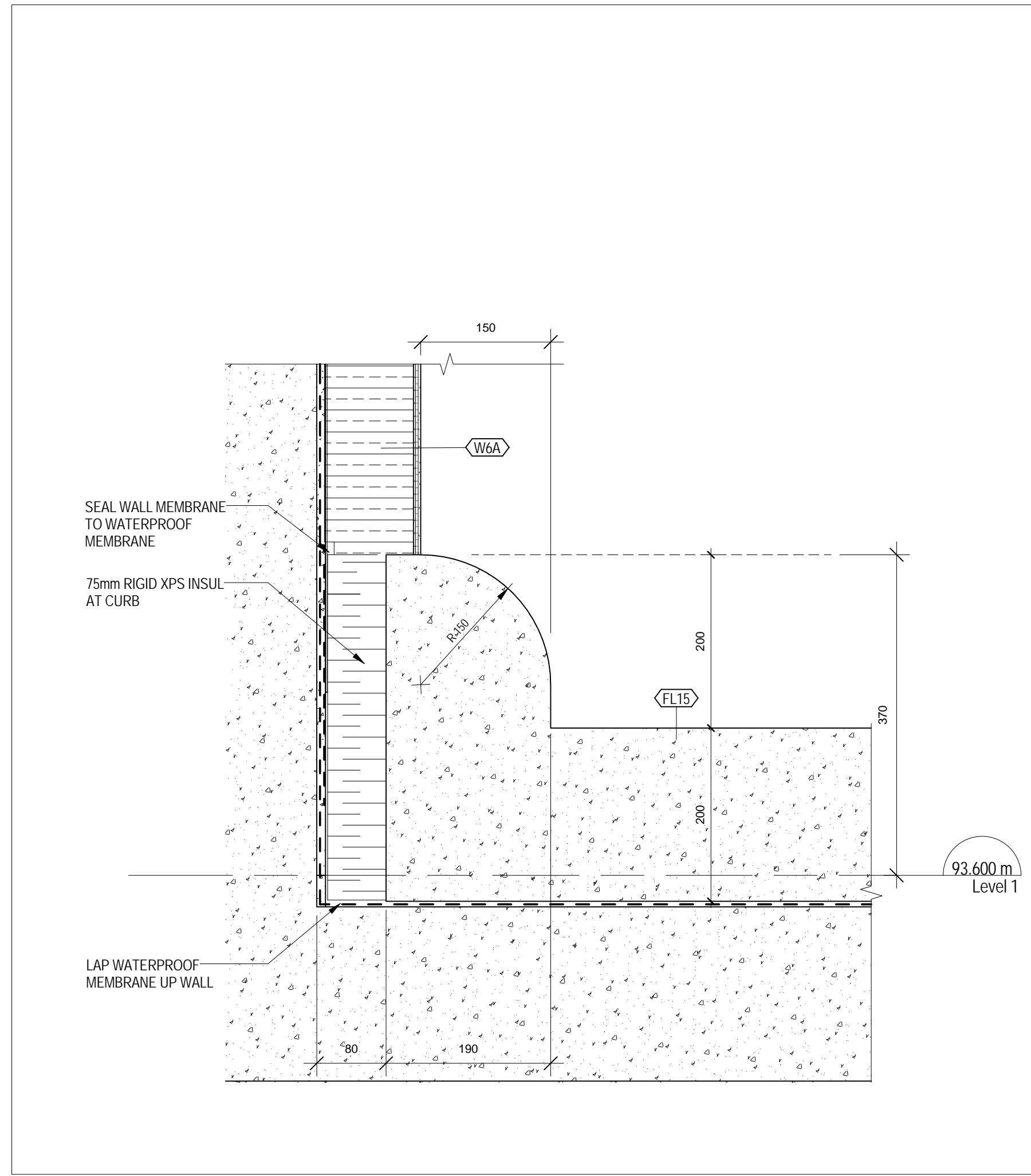
6 A 610 1:5 LOADING DOCK CURB WEST WALL
