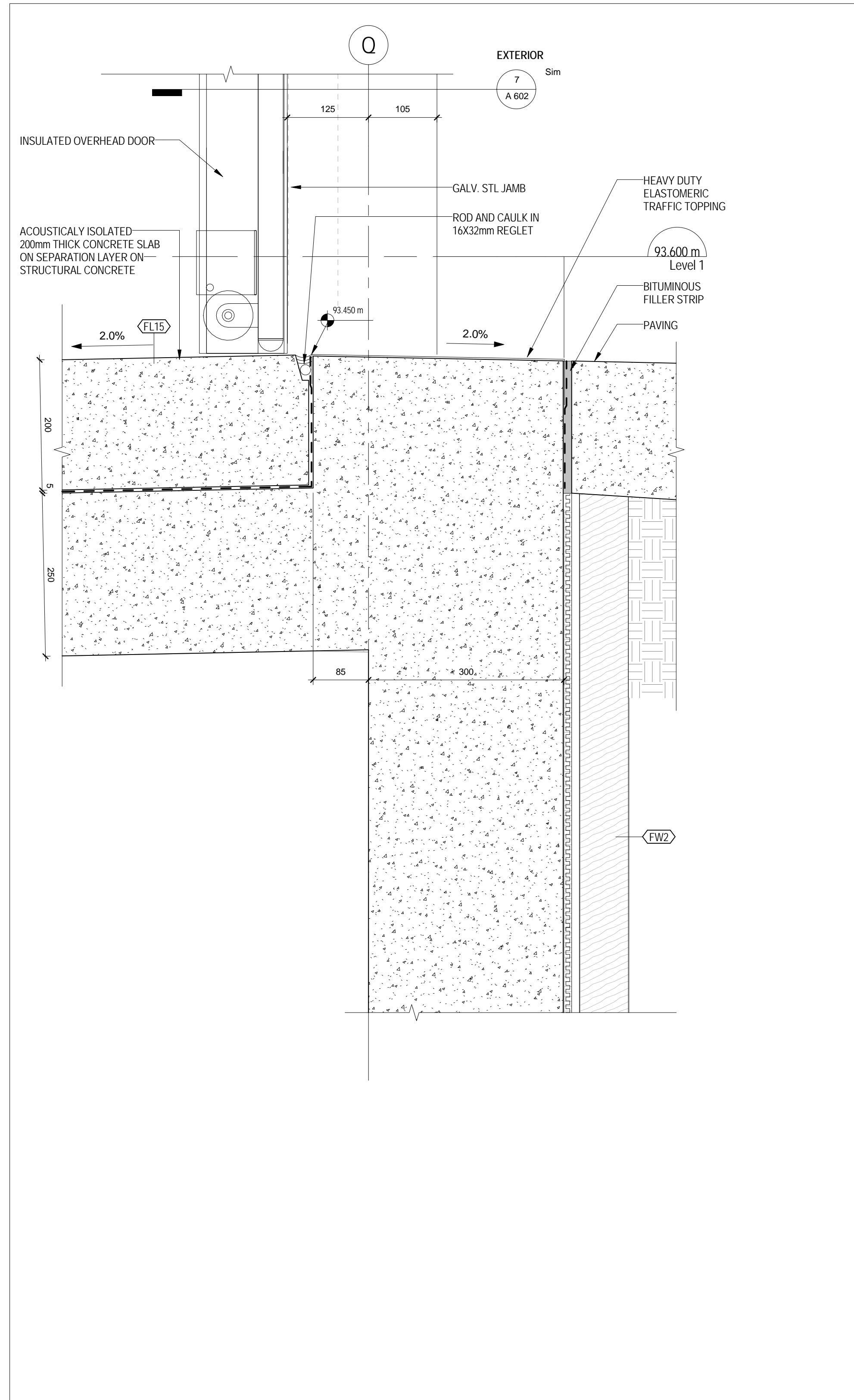
3 A 610 1:5 FOUNDATION WALL AT LOADING
