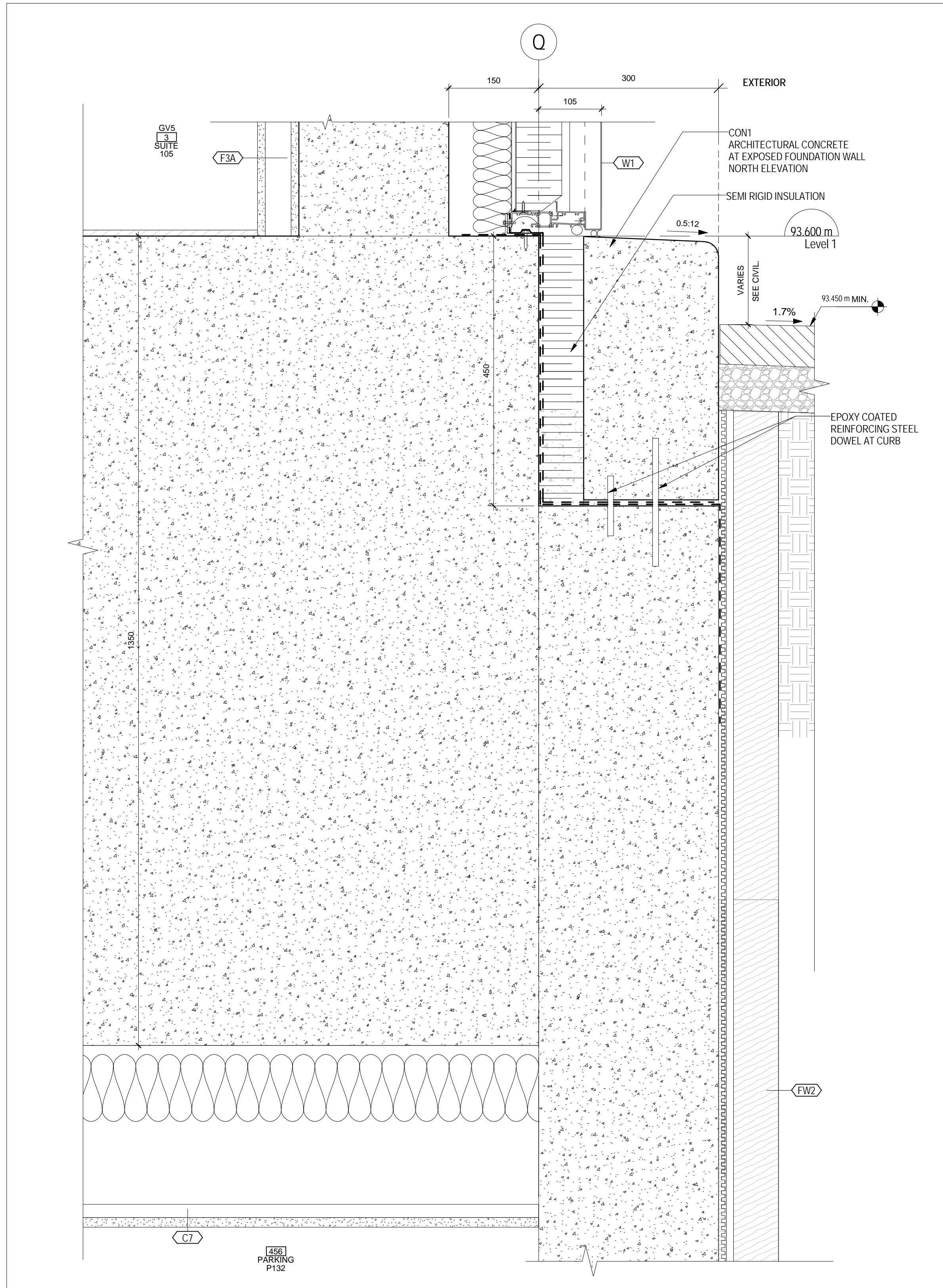
4 A 610 1:5 FOUNDATION WALL AT TOWNHOUSE
