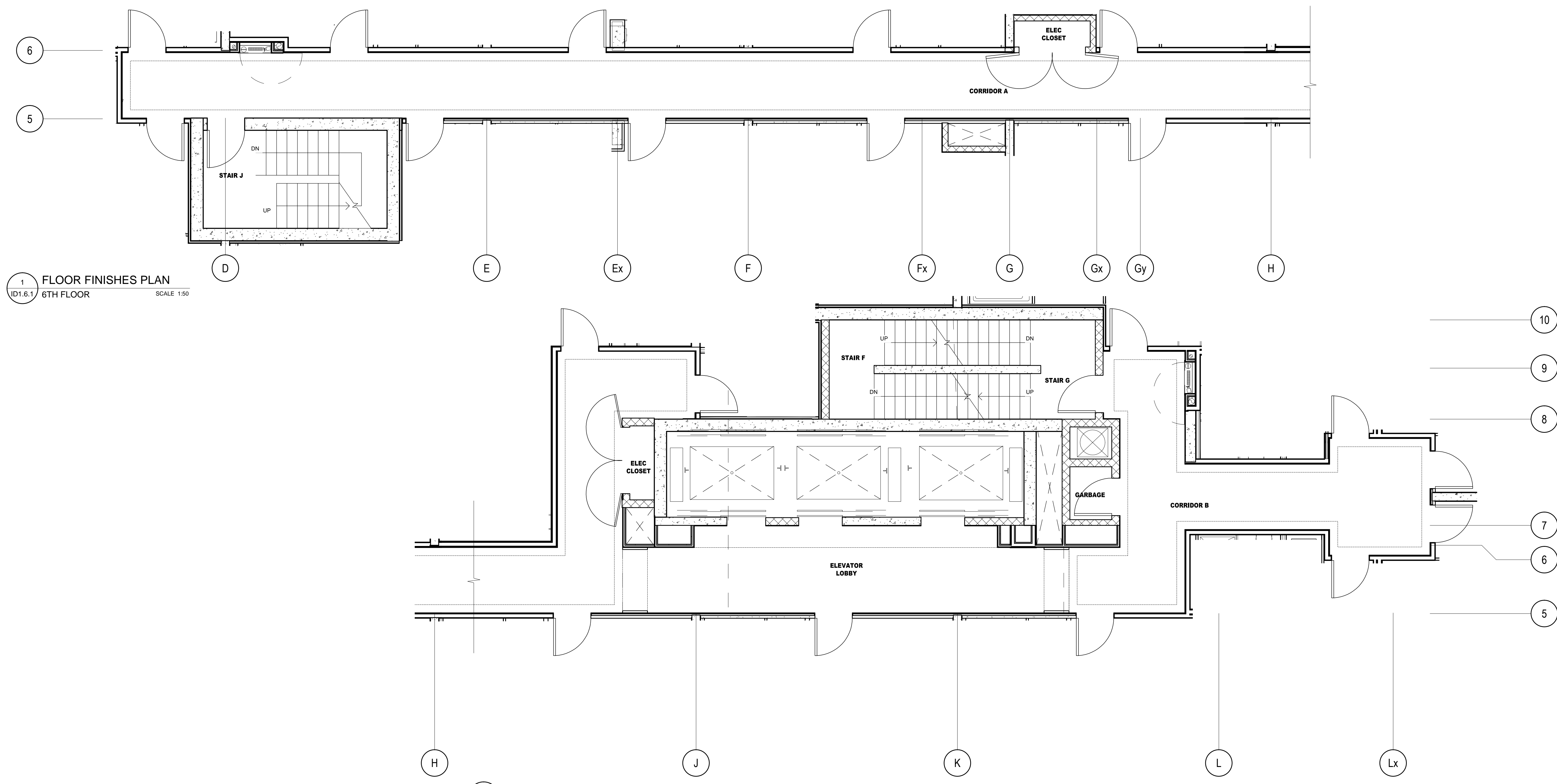
2 FLOOR FINISHES PLAN 6TH FLOOR SCALE 1:50
