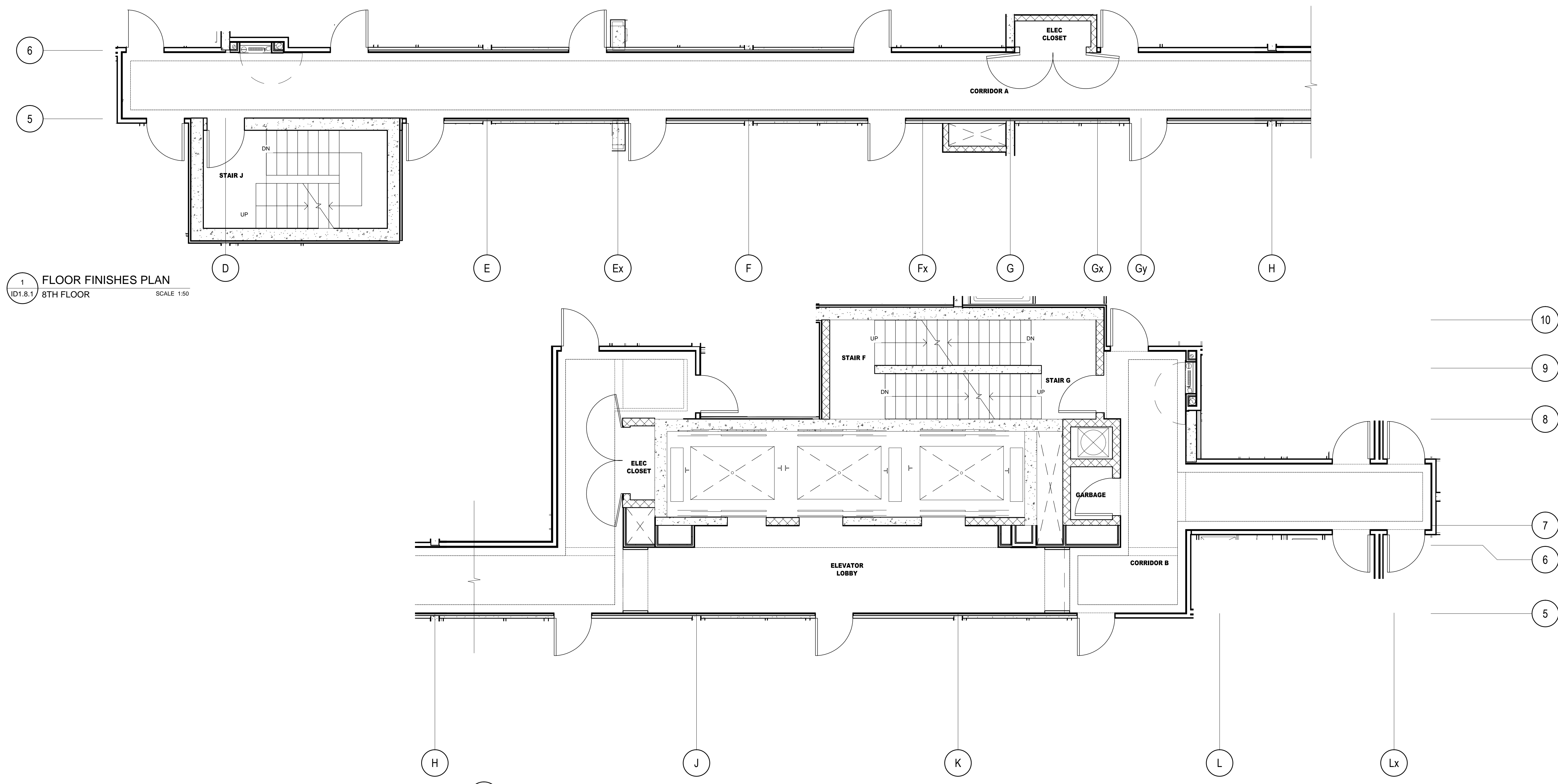
2 FLOOR FINISHES PLAN 8TH FLOOR SCALE 1:50
