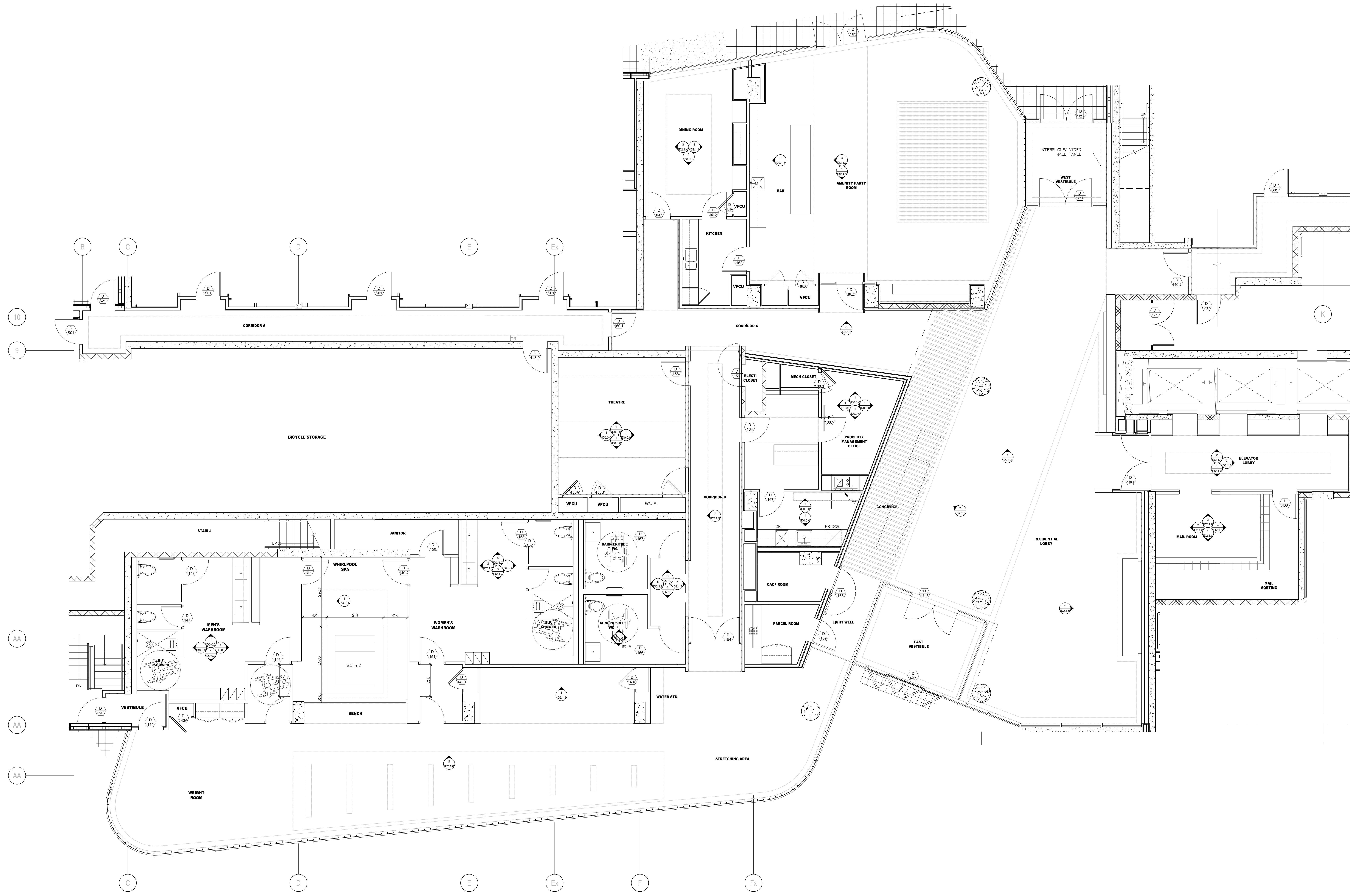
1 CONSTRUCTION PLAN ID1.1.0 GROUND FLOOR SCALE 1:50
