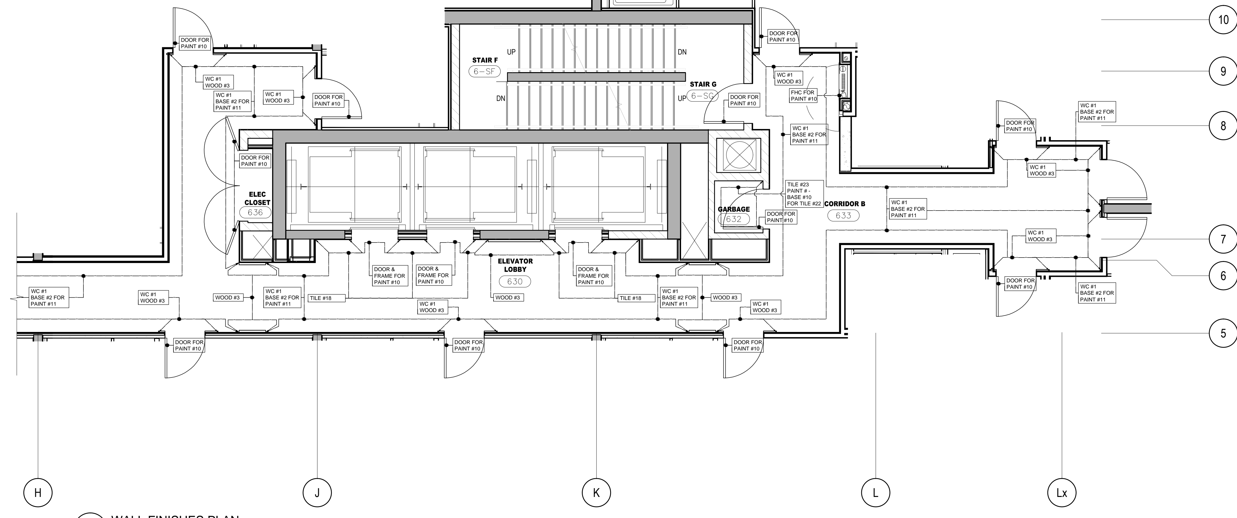
4 WALL FINISHES PLAN 6TH FLOOR SCALE 1:50
