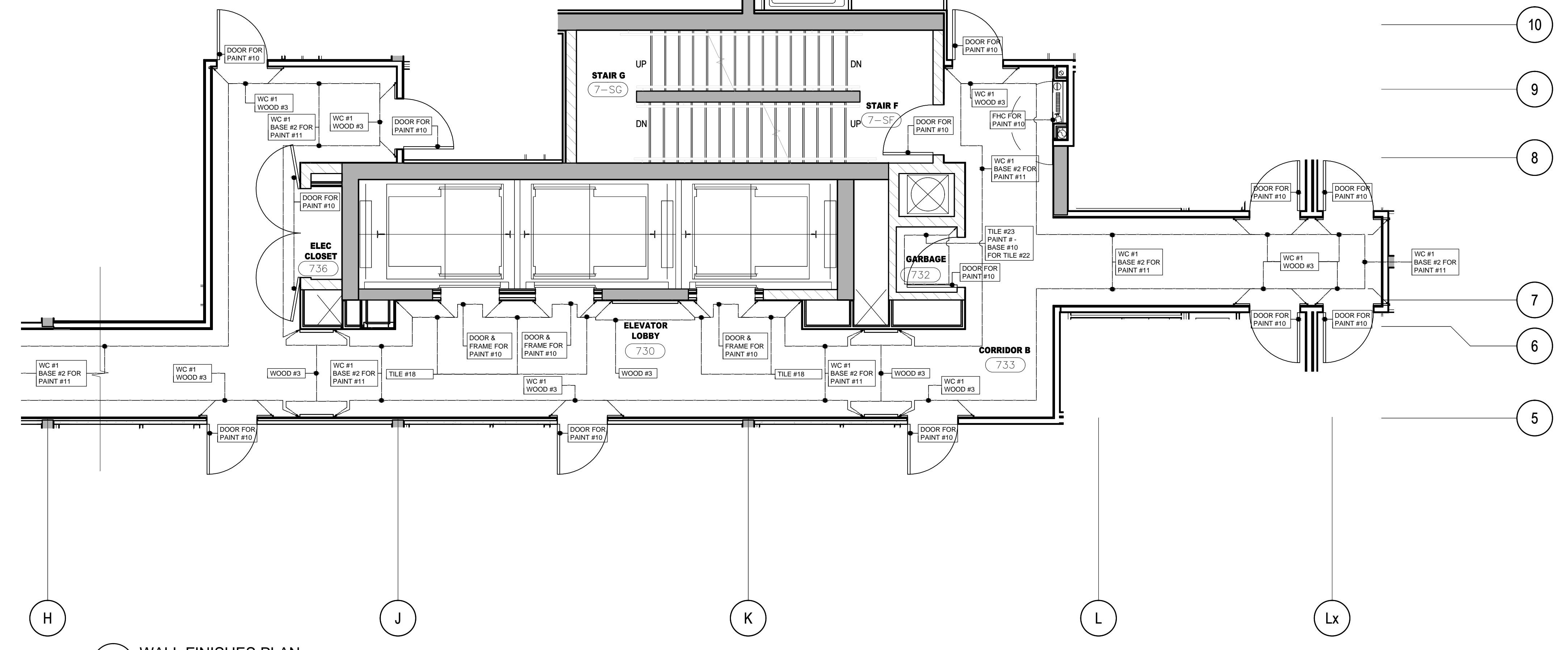
4 WALL FINISHES PLAN ID1.7.1 7TH FLOOR SCALE 1:50
