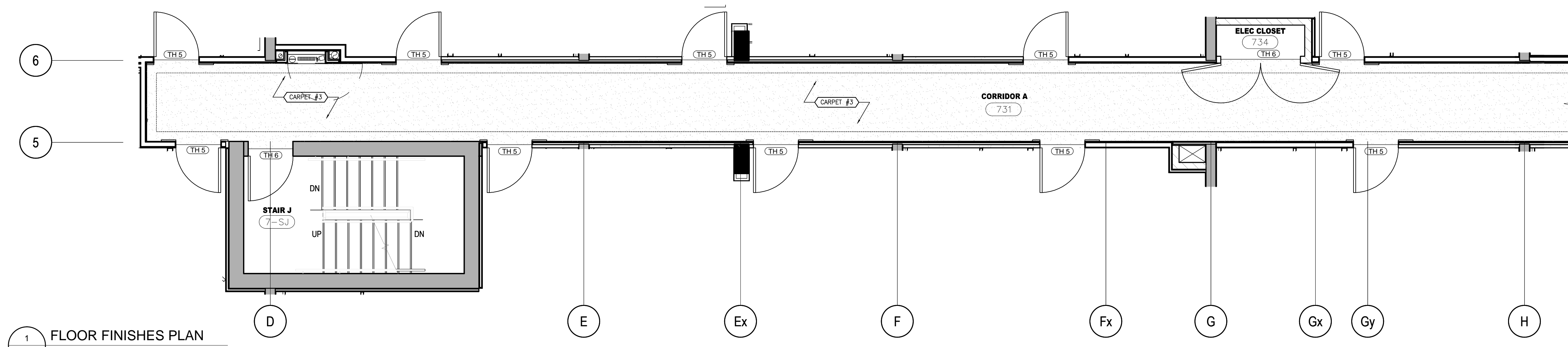
1 FLOOR FINISHES PLAN ID1.7.1 7TH FLOOR SCALE 1:50
