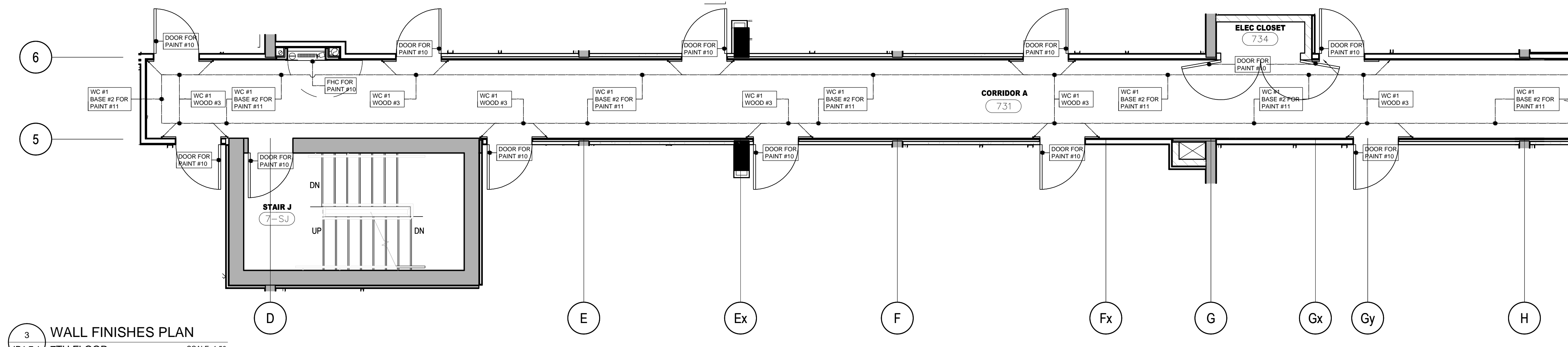
3 WALL FINISHES PLAN ID1.7.1 7TH FLOOR SCALE 1:50
