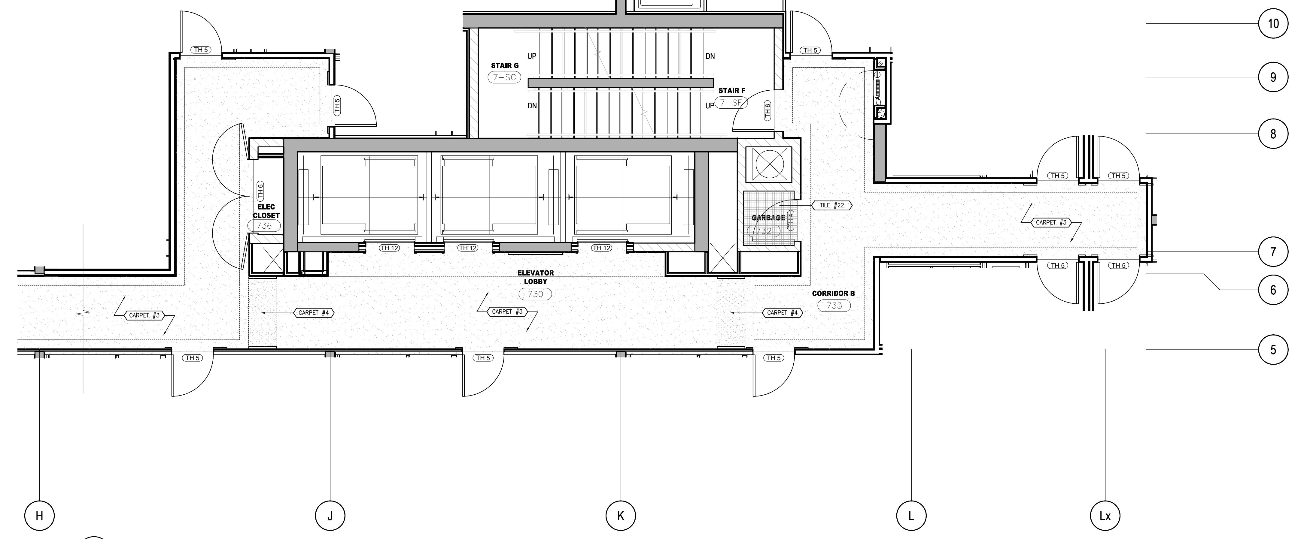
2 FLOOR FINISHES PLAN ID1.7.1 7TH FLOOR SCALE 1:50
