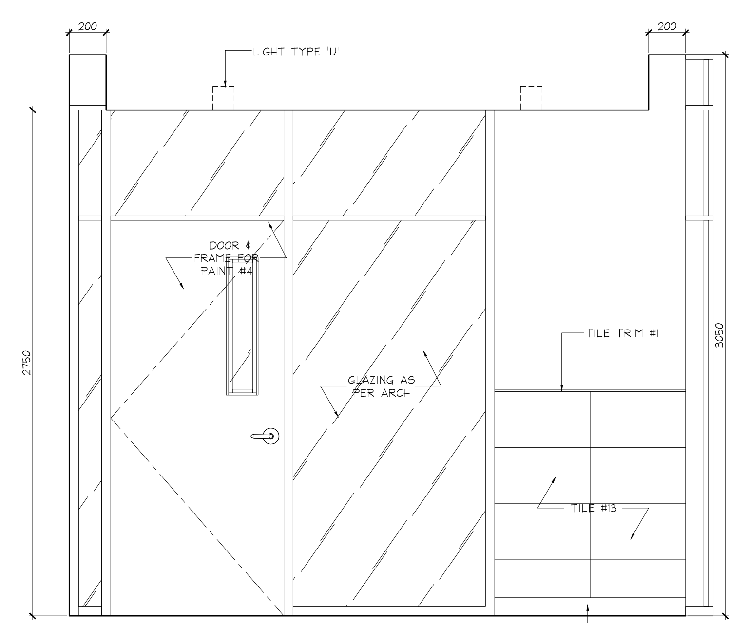
7 ELEVATION ID2.0.1 P1 LEVEL VESTIBULE SCALE 1:20
