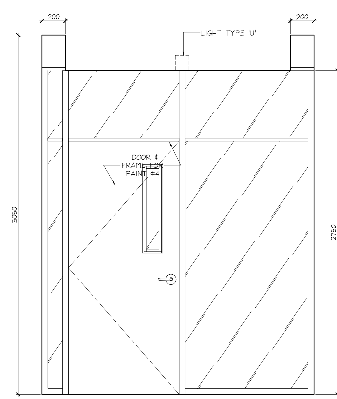
5 ELEVATION ID2.0.1 P1 LEVEL VESTIBULE SCALE 1:20
