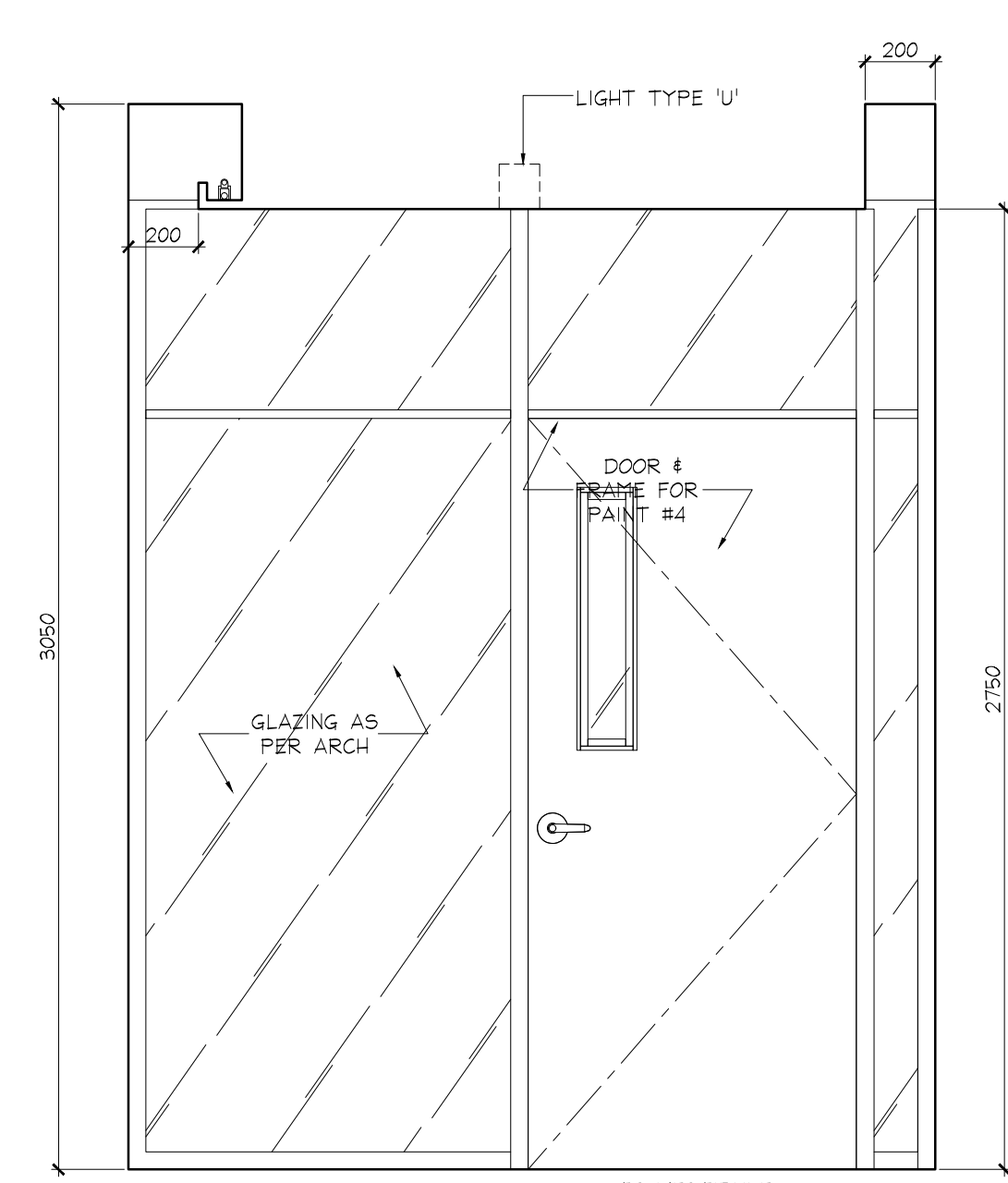
3 ELEVATION ID2.0.1 P1 LEVEL ELEVATOR LOBBY SCALE 1:20
