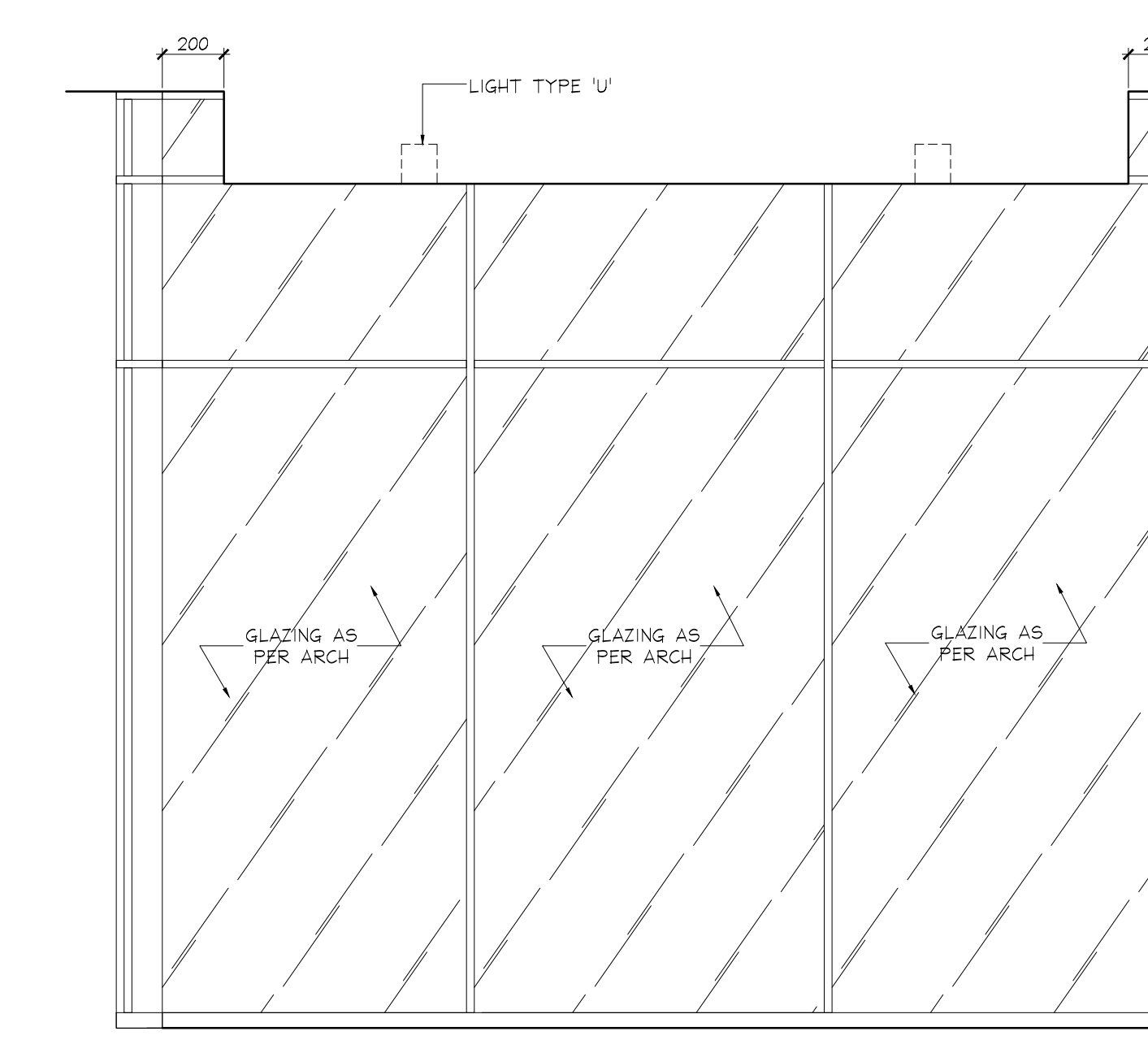
8 ELEVATION ID2.0.1 P1 LEVEL VESTIBULE SCALE 1:20
