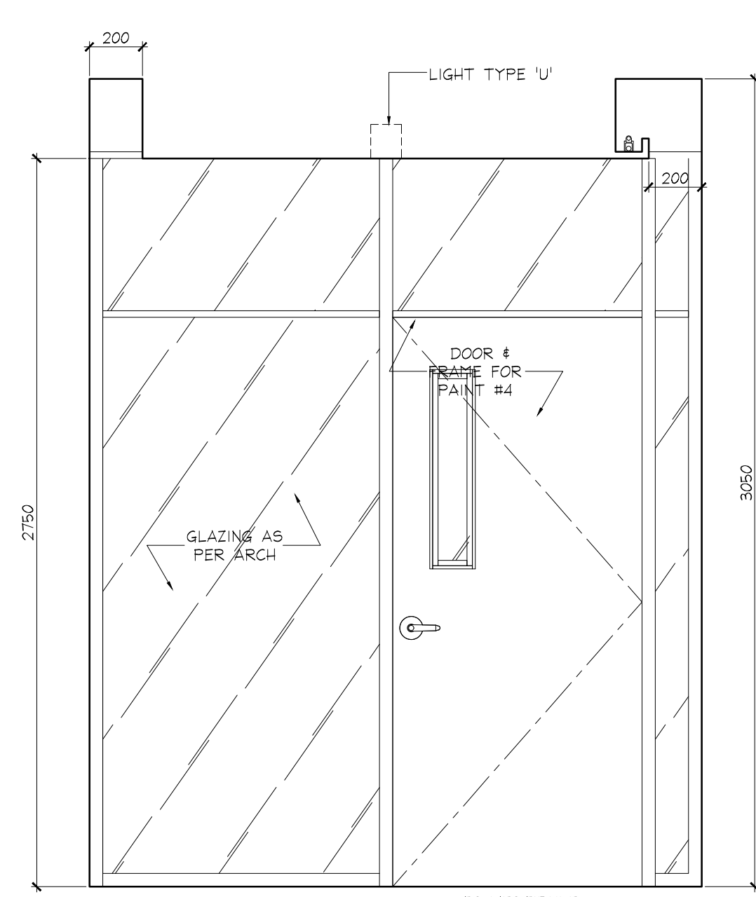
4 ELEVATION ID2.0.1 P1 LEVEL ELEVATOR LOBBY SCALE 1:20
