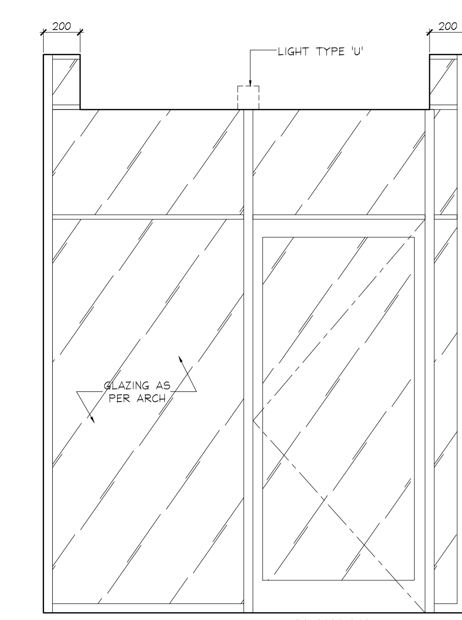
6 ELEVATION ID2.0.1 P1 LEVEL VESTIBULE SCALE 1:20
