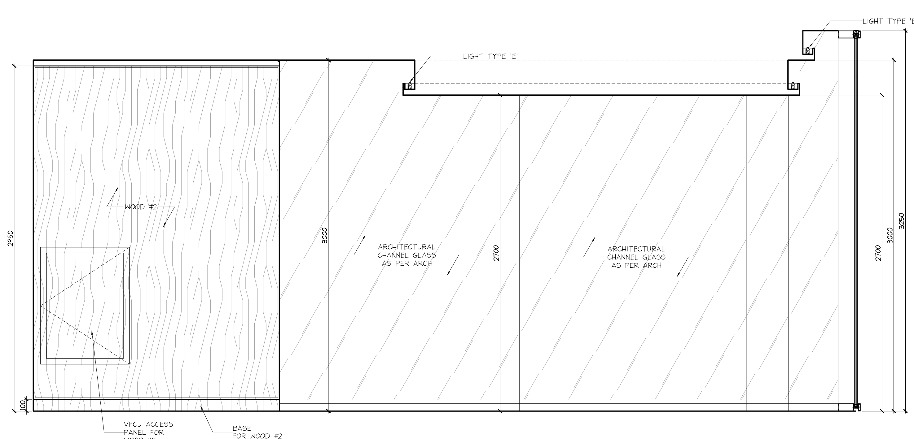
3 ELEVATION 102.1.6 GROUND FLOOR WEIGHT ROOM SCALE 1:20
