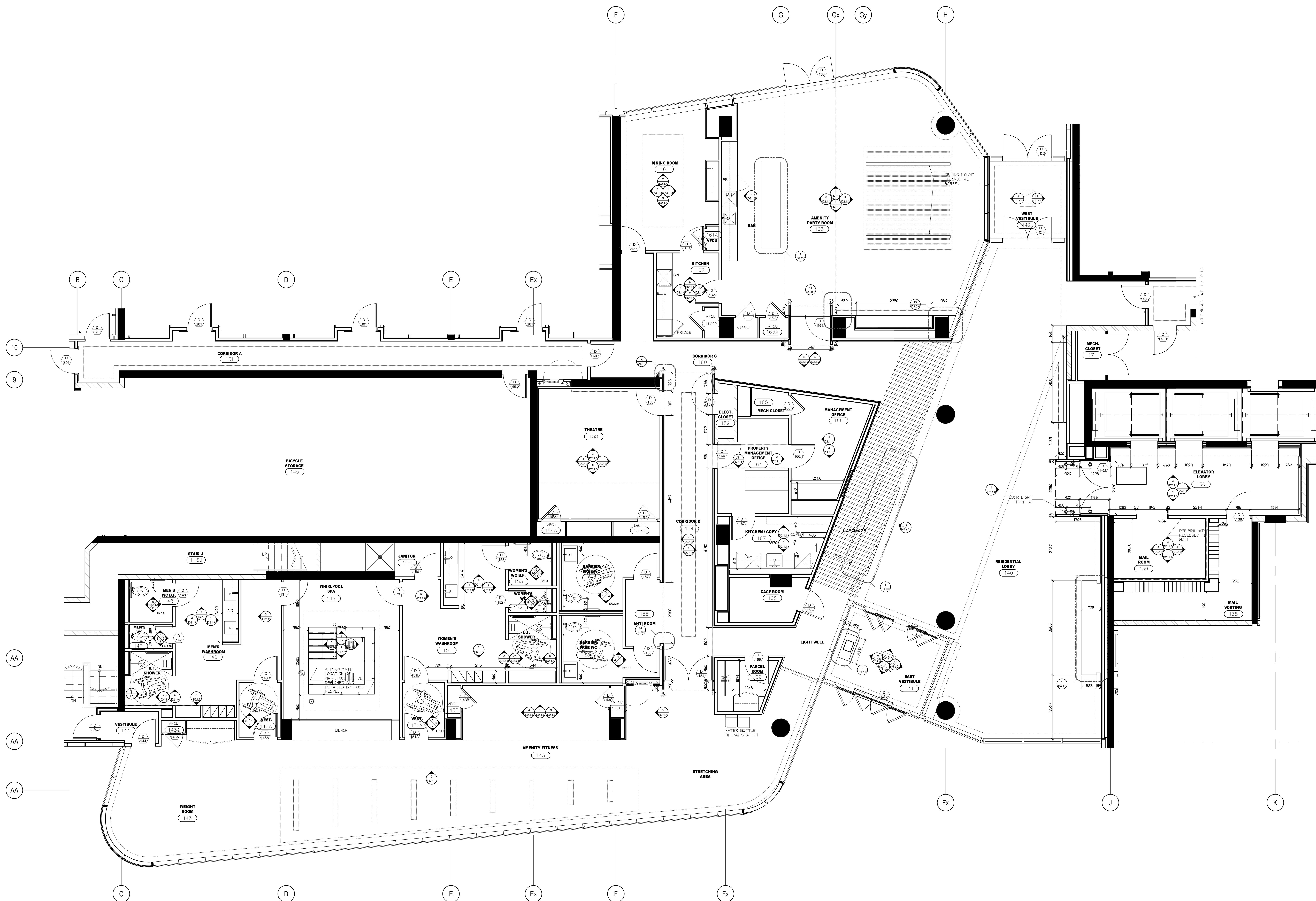
1 CONSTRUCTION PLAN 101.1.0 GROUND FLOOR SCALE 1:50
