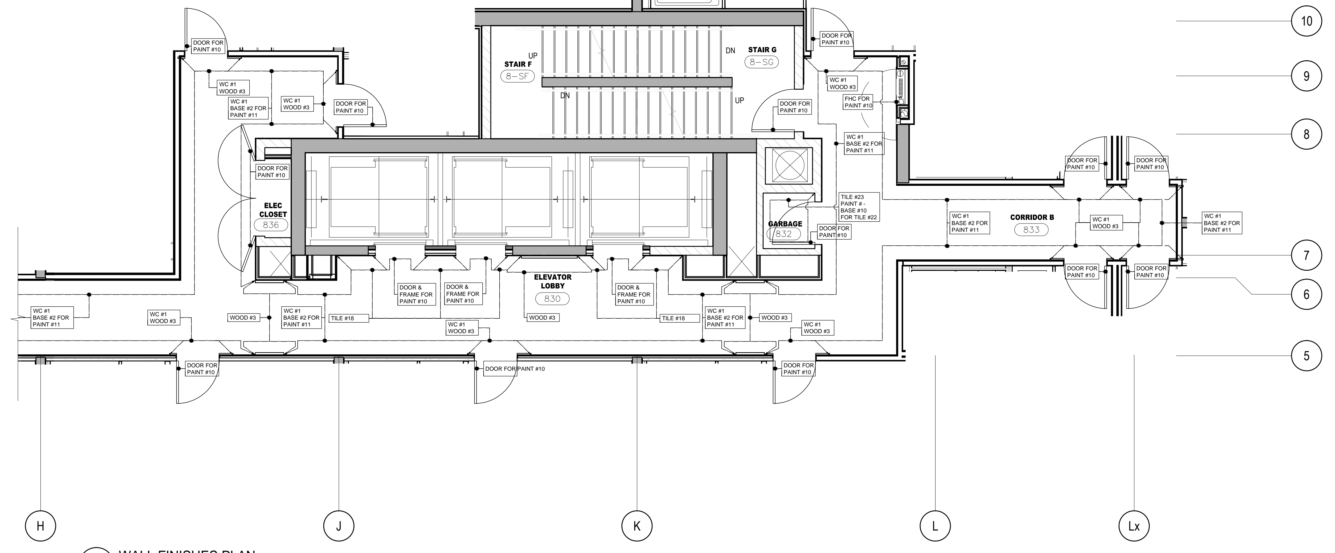
4 WALL FINISHES PLAN 8TH FLOOR SCALE 1:50
