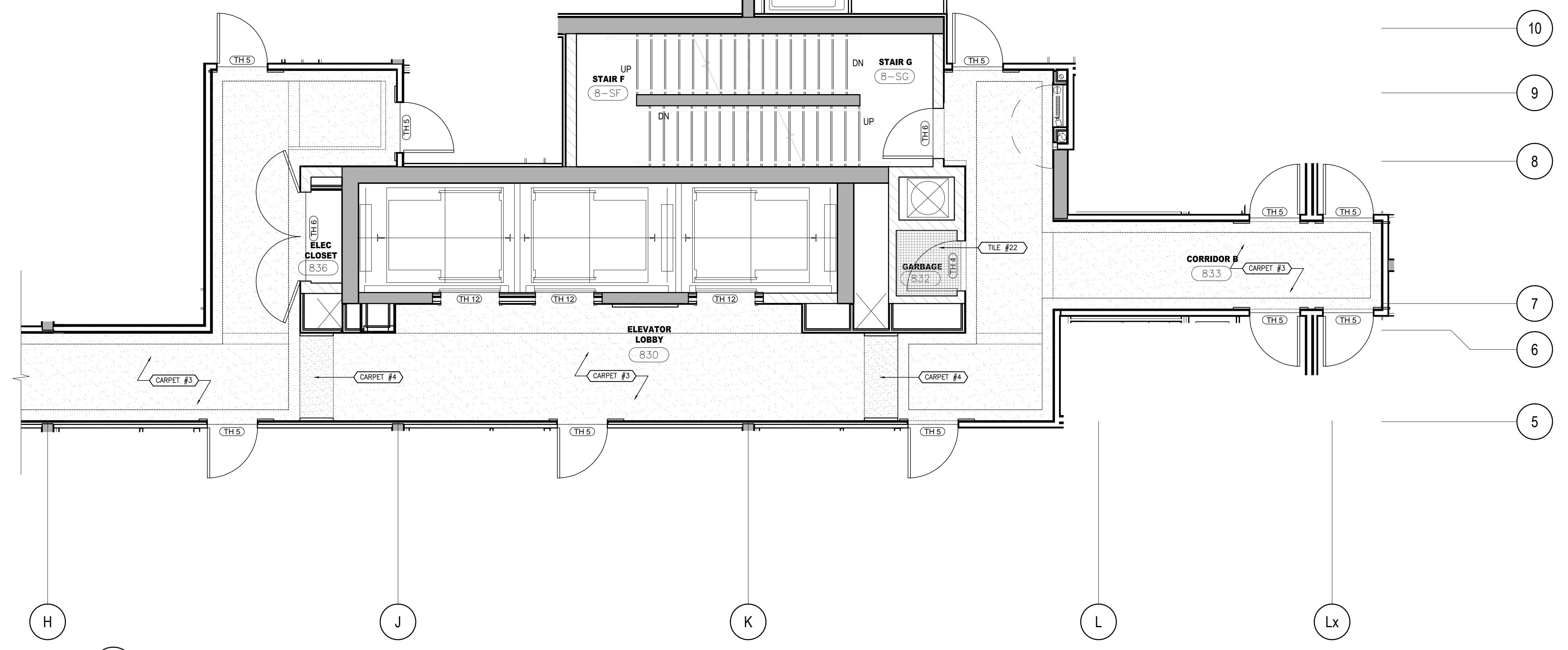
2 FLOOR FINISHES PLAN 8TH FLOOR SCALE 1:50
