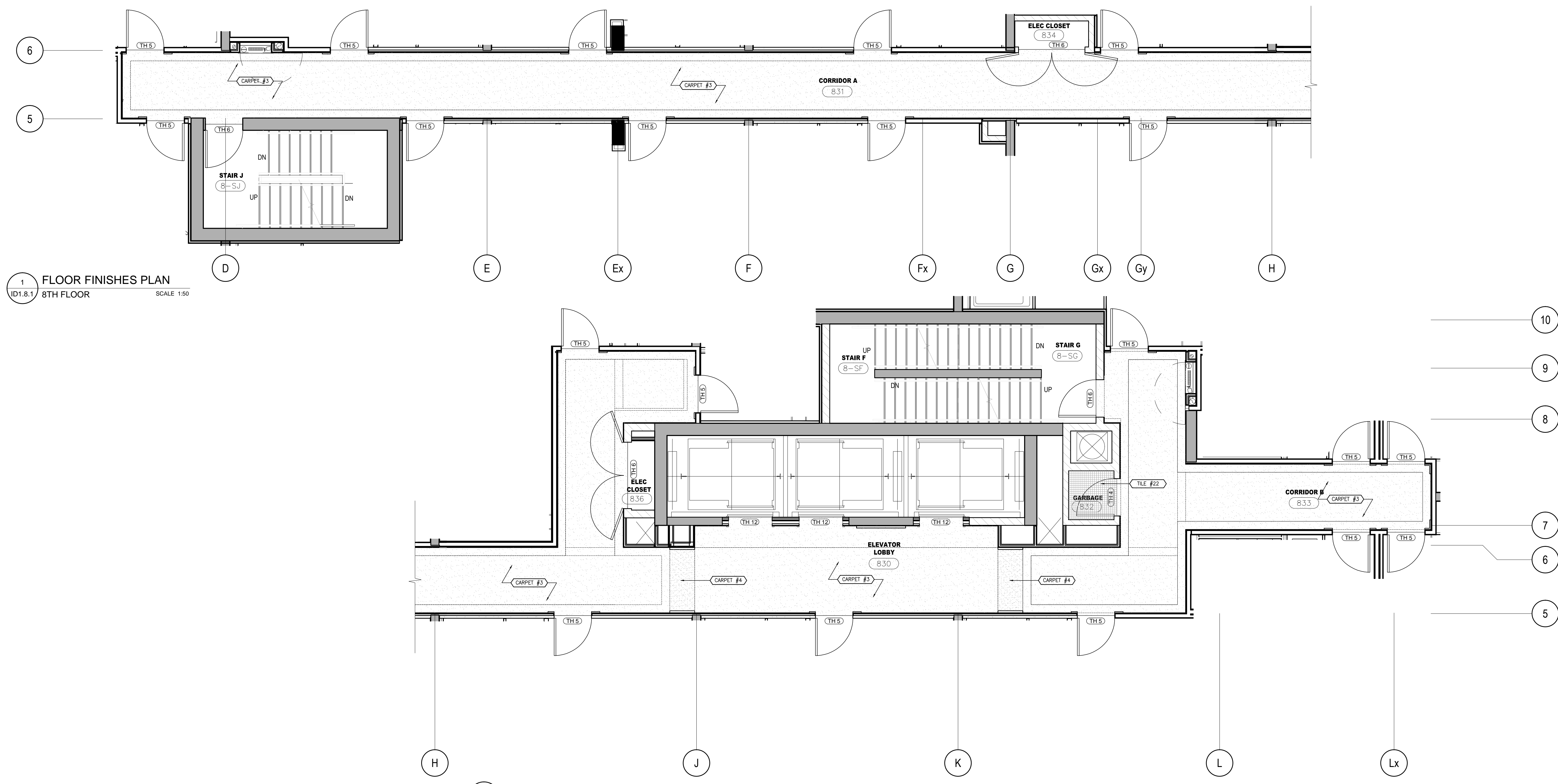
2 FLOOR FINISHES PLAN ID1.8.1 8TH FLOOR SCALE 1:50
