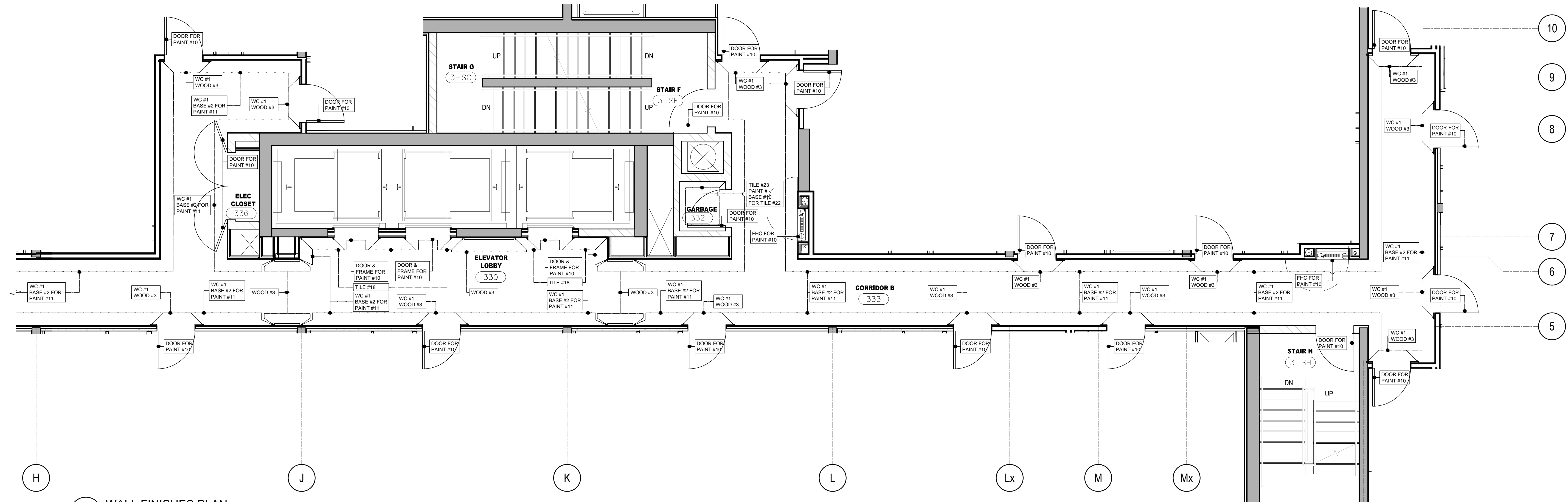
4 WALL FINISHES PLAN 3RD FLOOR SCALE 1:50 ID1.3.1
