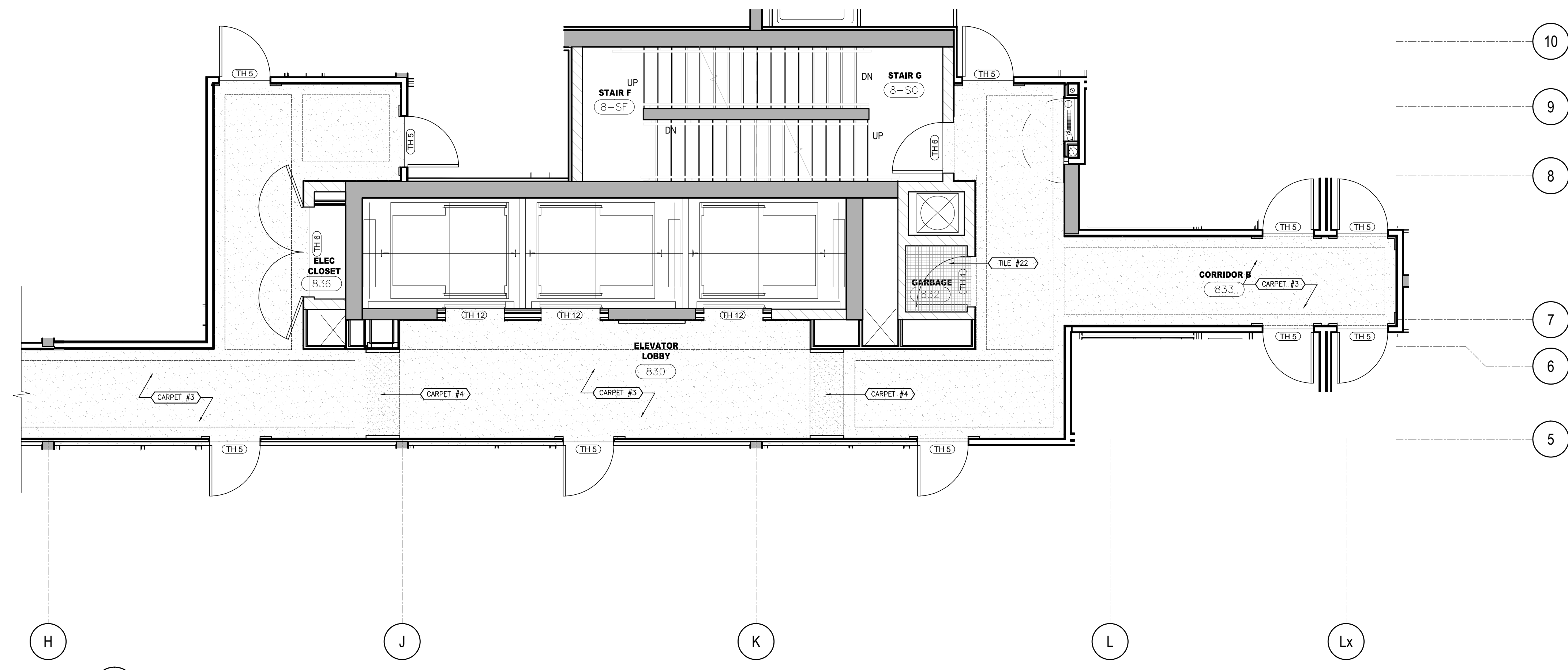
2 FLOOR FINISHES PLAN 8TH FLOOR SCALE 1:50
