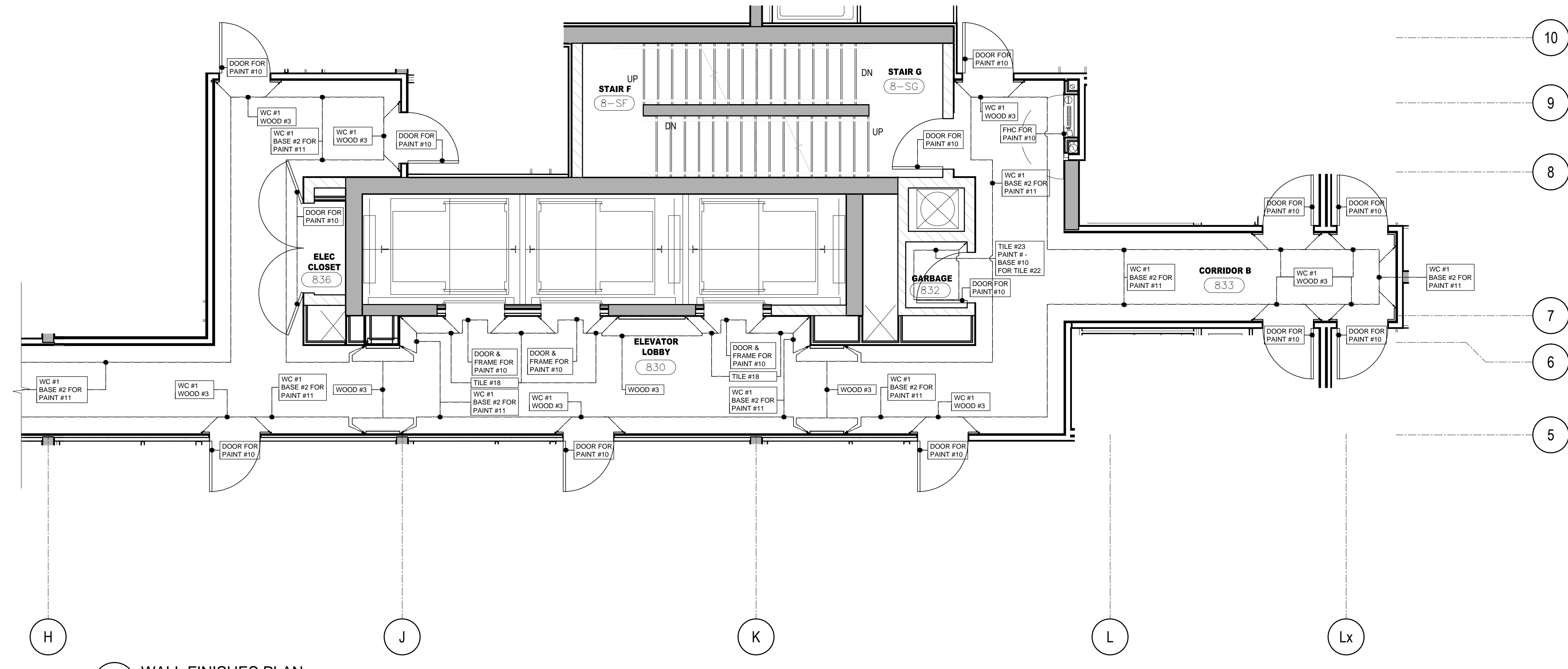
4 WALL FINISHES PLAN 8TH FLOOR SCALE 1:50
