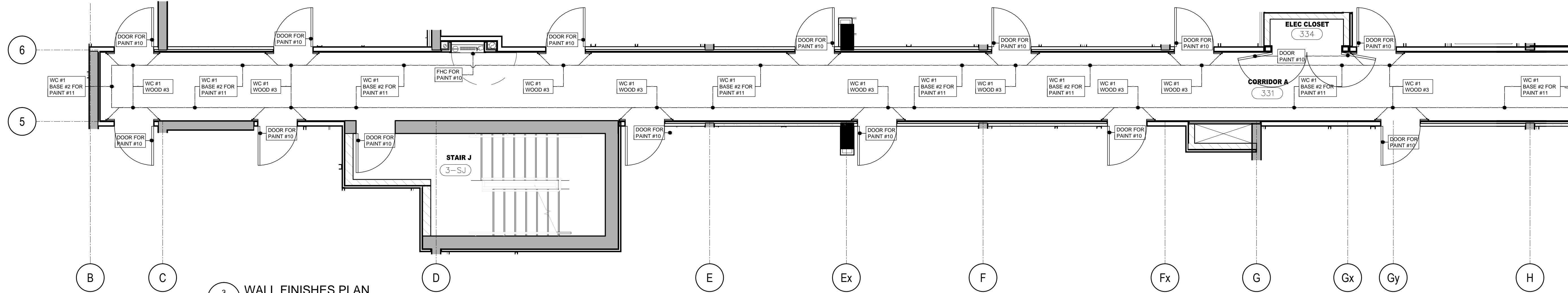
3 WALL FINISHES PLAN 3RD FLOOR SCALE 1:50 IDI.3.1
