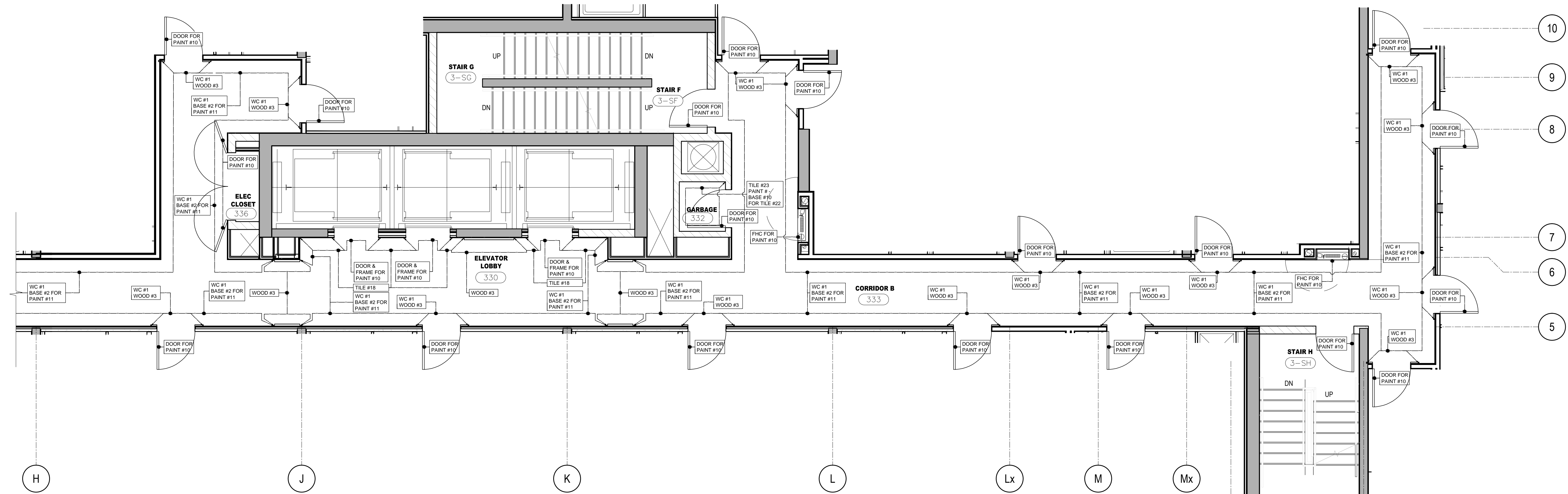
4 WALL FINISHES PLAN 3RD FLOOR SCALE 1:50 IDI.3.1
