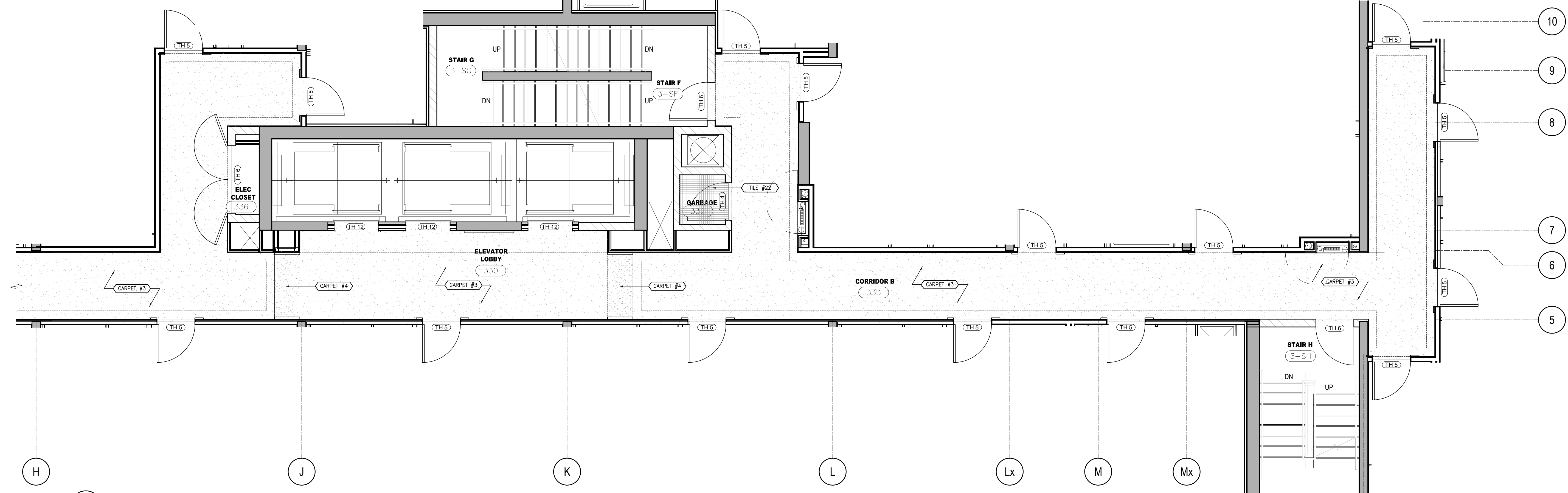
2 FLOOR FINISHES PLAN 3RD FLOOR SCALE 1:50 IDI.3.1
