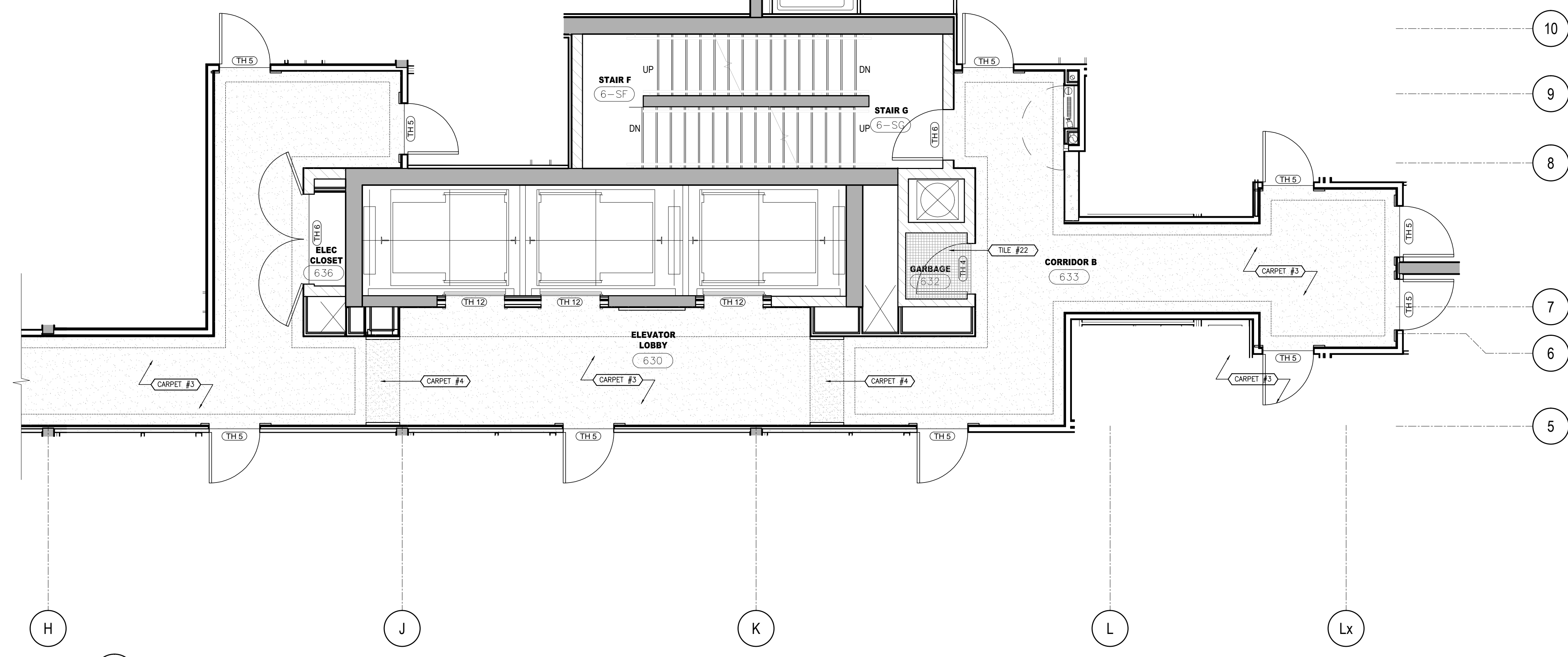
2 FLOOR FINISHES PLAN 6TH FLOOR SCALE 1:50
