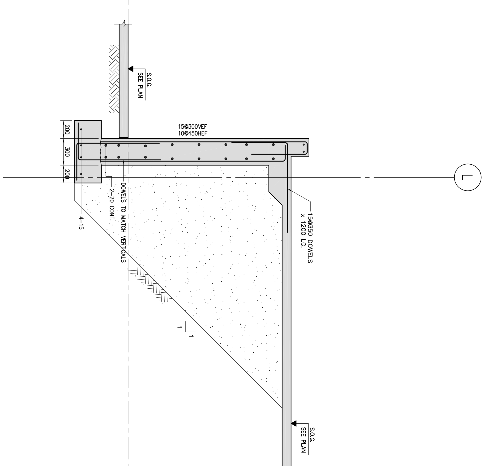
SECTION 3 SCALE 1:20 S-304
