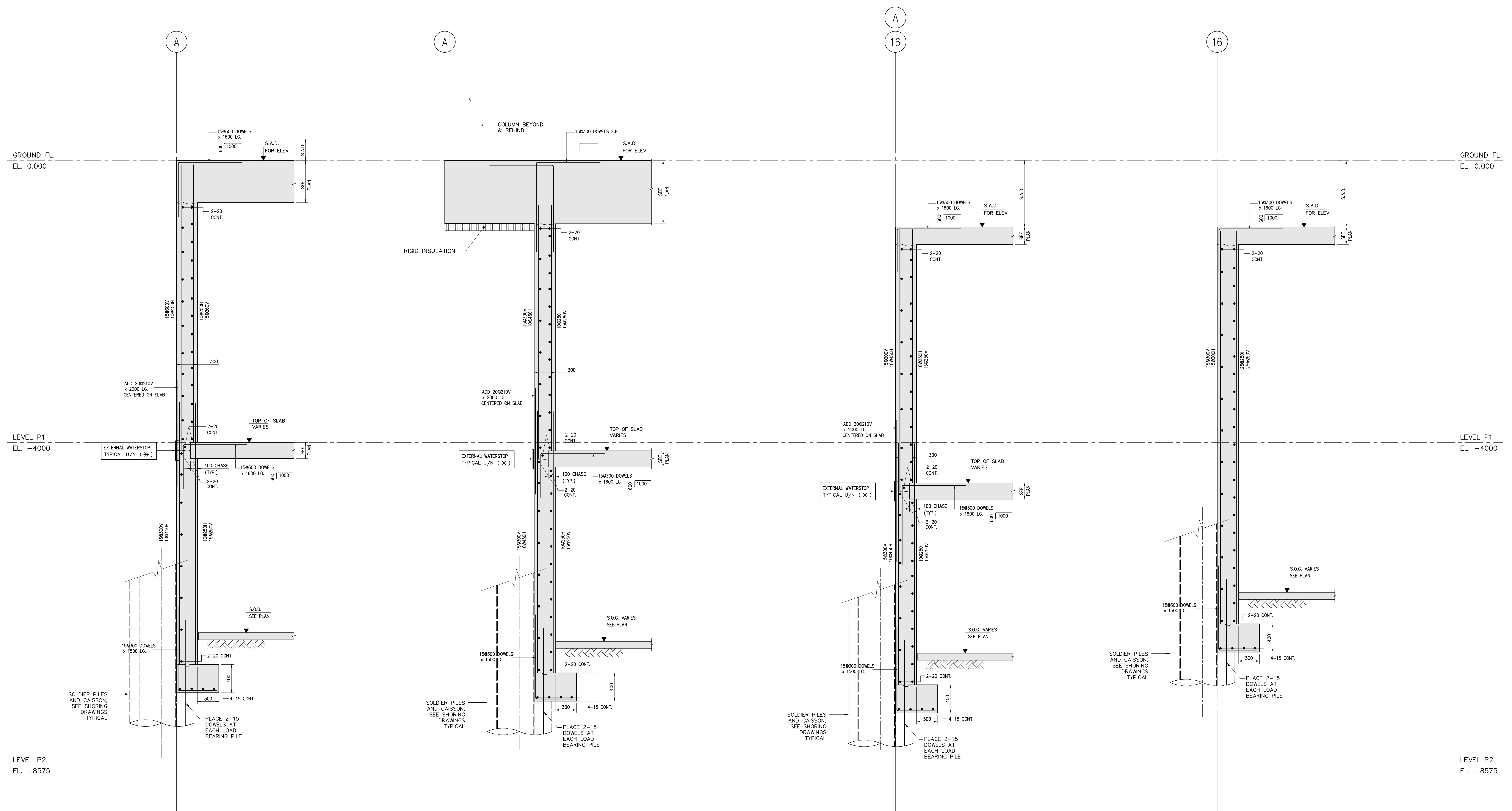
SECTION 1 SCALE 1:20
