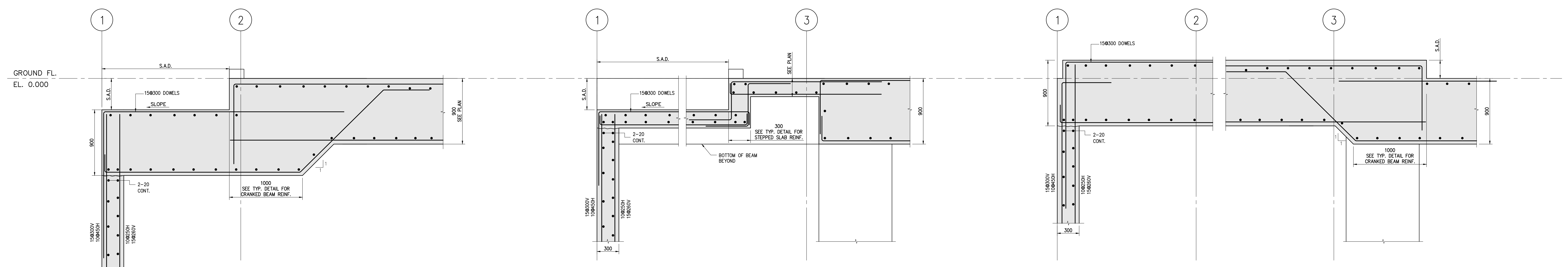
SECTION 5 SCALE 1:20
