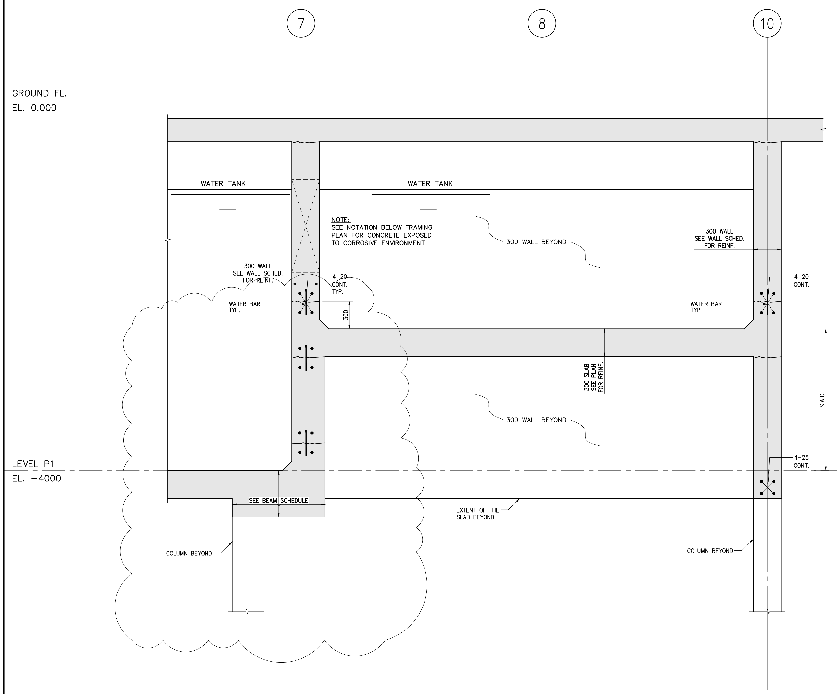
SECTION 3 SCALE 1:20
