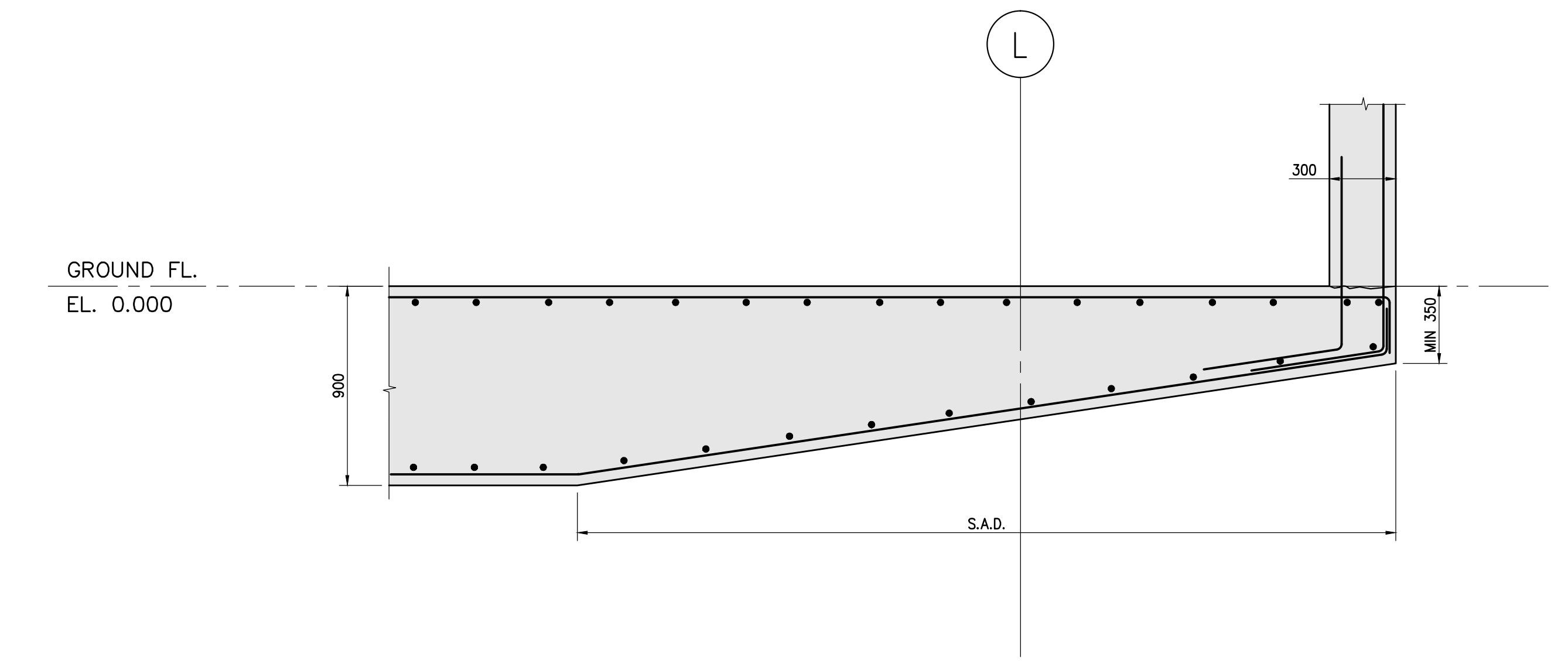
SECTION 5 SCALE 1:20
