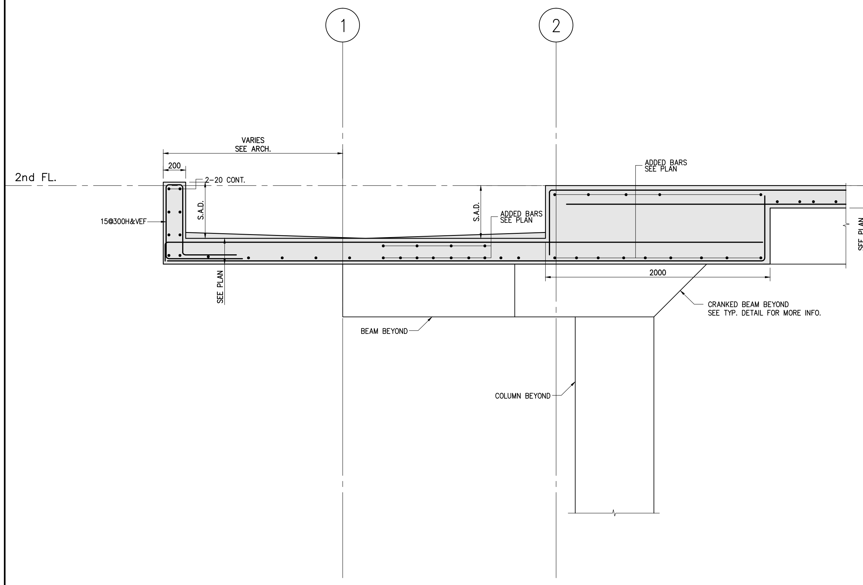
SECTION 1 SCALE 1:20
