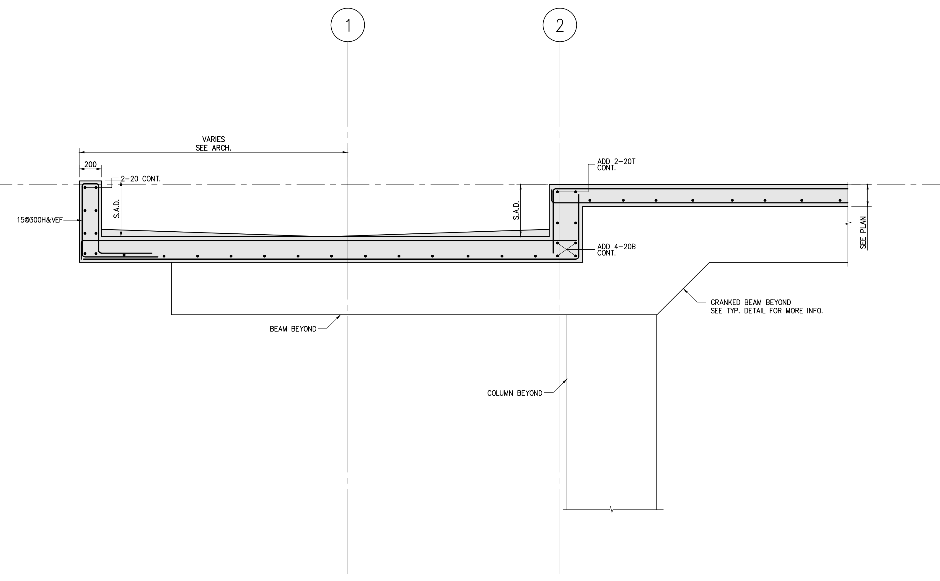
SECTION 2 SCALE 1:20
