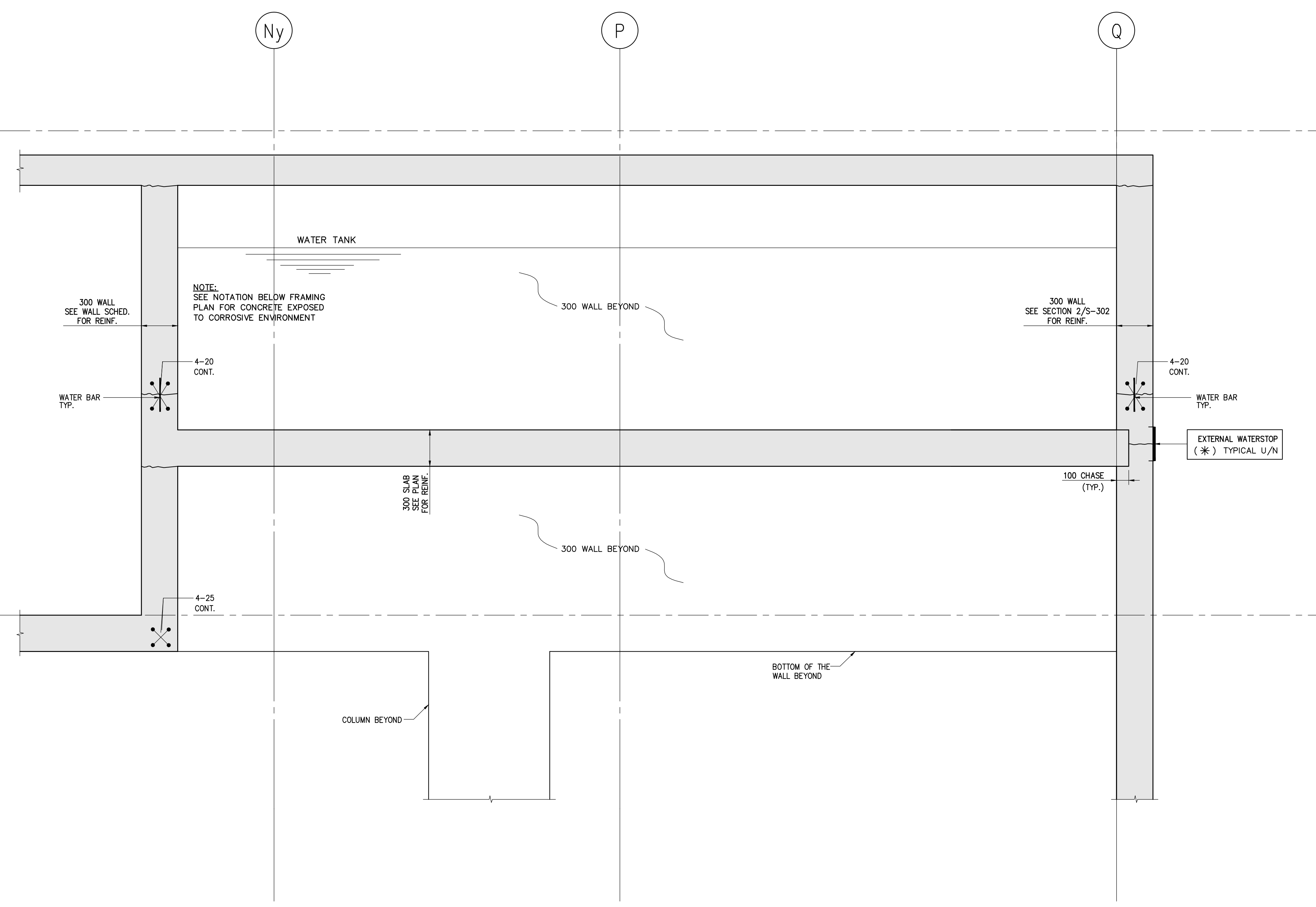
SECTION 4 SCALE 1:20
