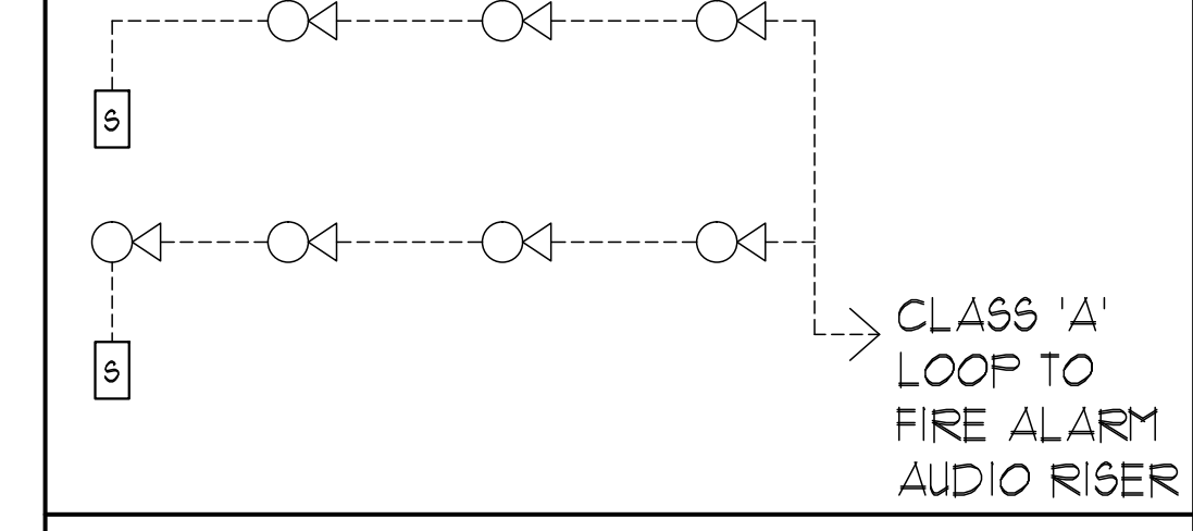
SUITE FIRE ALARM SYSTEM CONNECTION DIAGRAM
