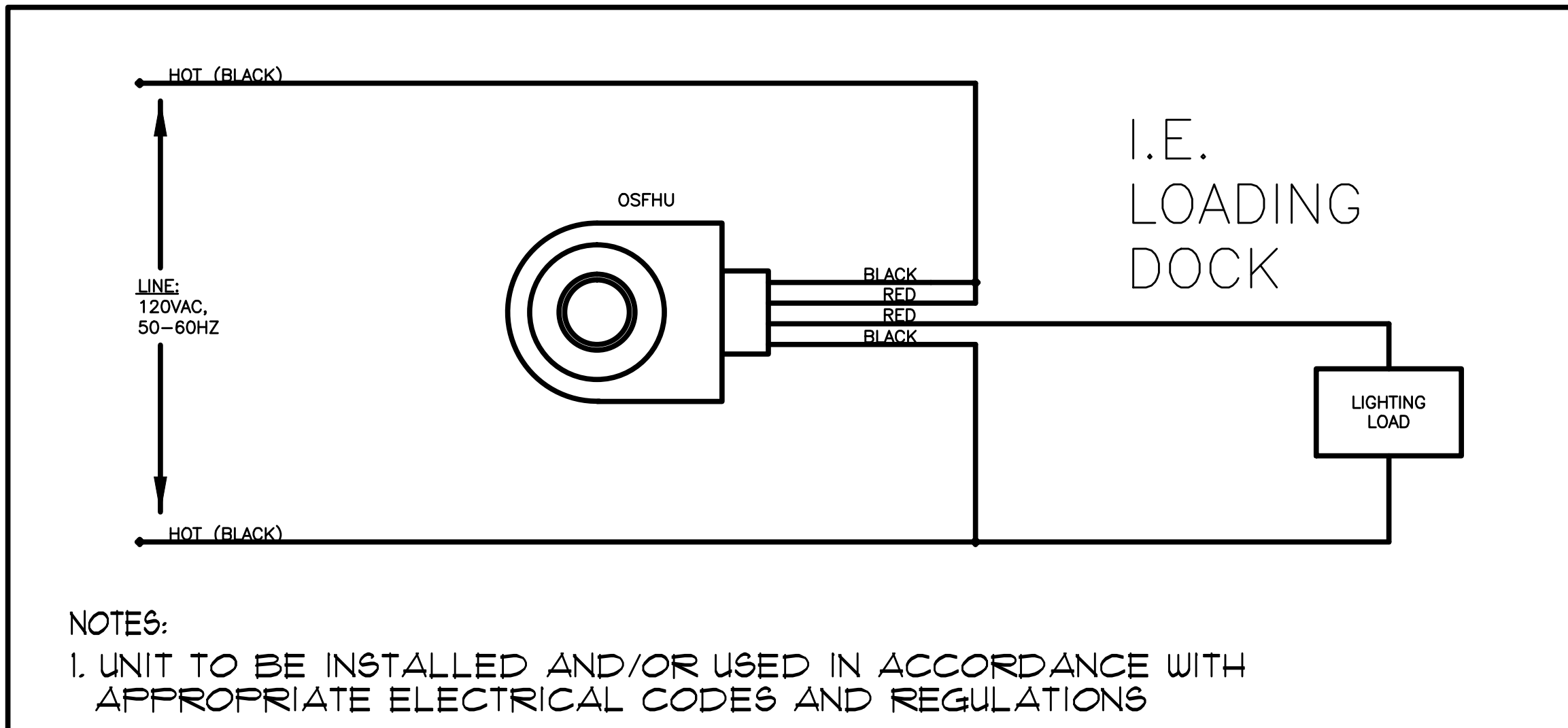
DETAIL 'A' FIXTURE MOUNTED HI-BAY/LOW-BAY PIR OCCUPANCY SENSOR SCALE: N.T.S.
