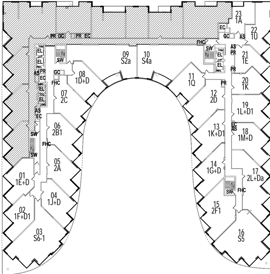
FLOOR 5
