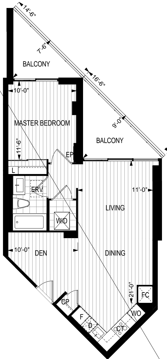
PARTIAL BALCONY PLAN: LEVELS 8, 10 1B+D1
