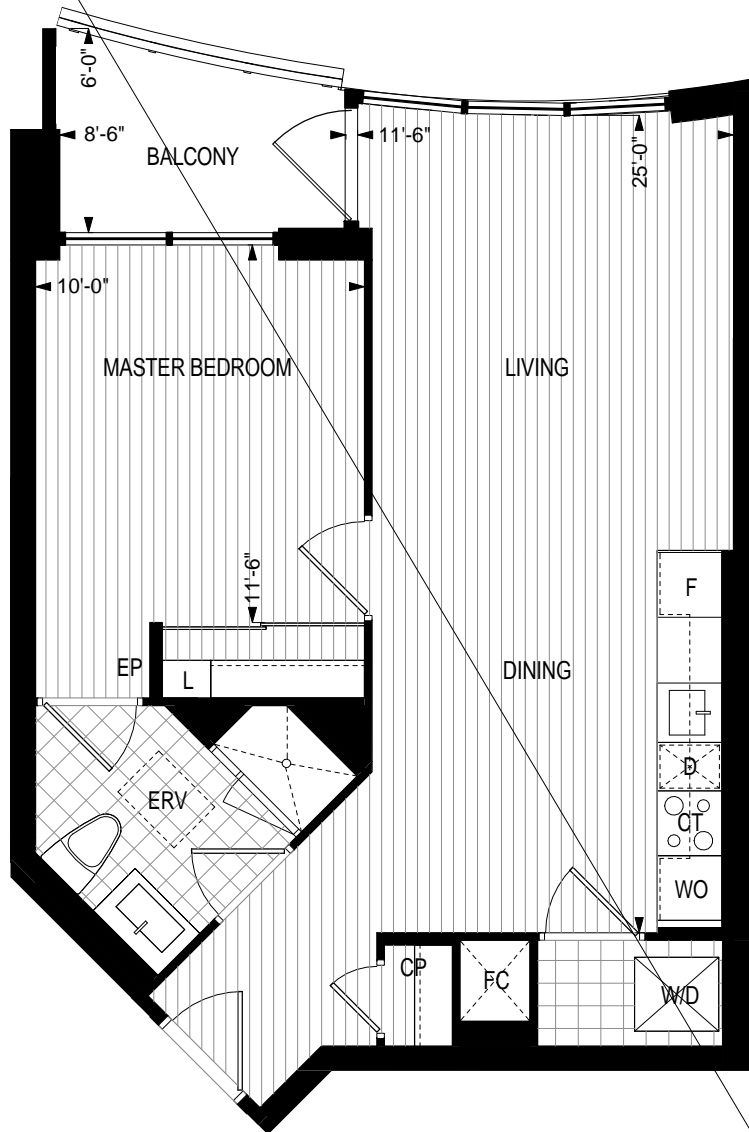
BALCONY PLAN: LEVELS 3, 6
