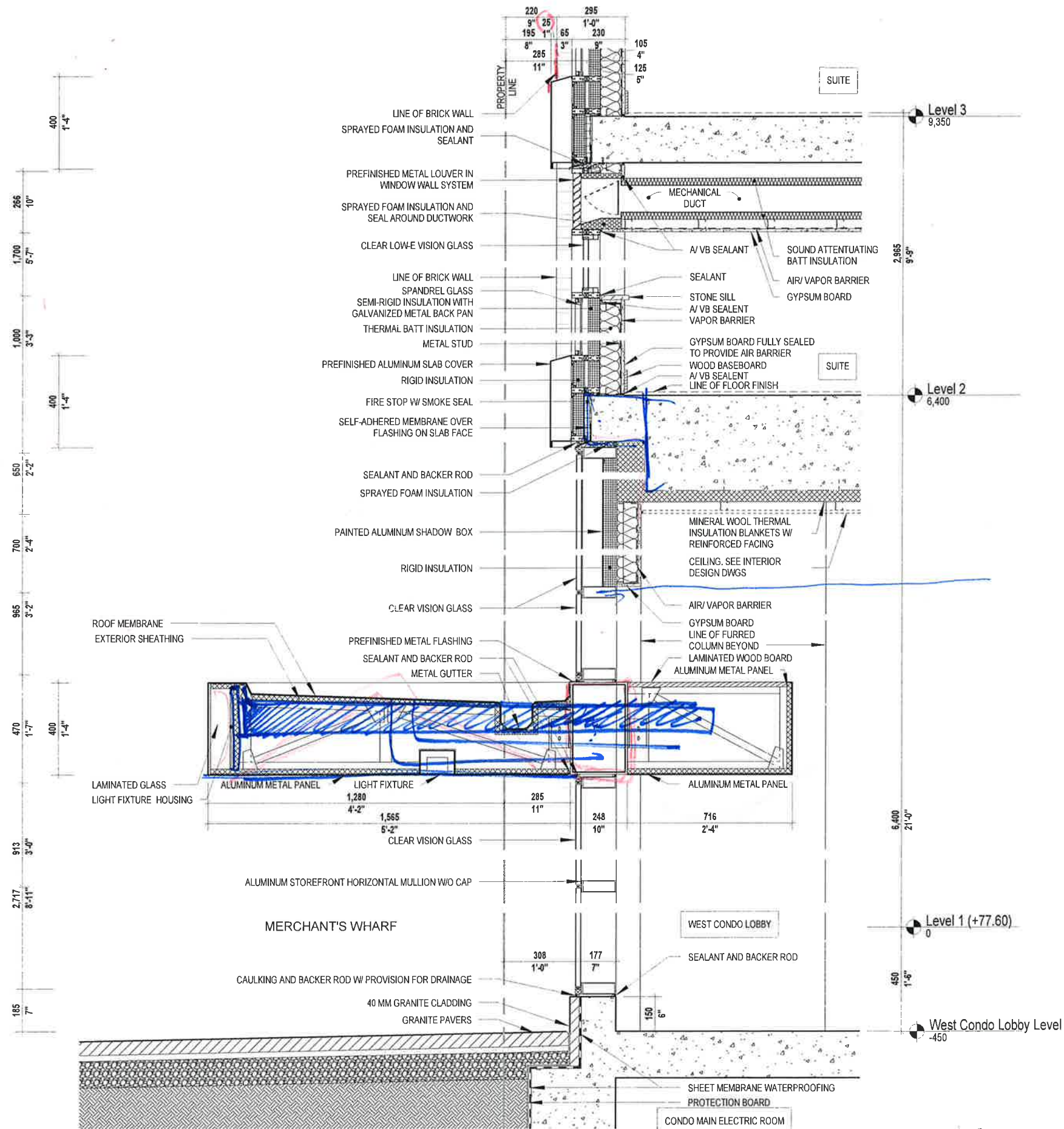
SECTION DETAIL - STOREFRONT - MULLIONS W/O CAPS AT CANOPY 1 1 : 20 EG.1.2
