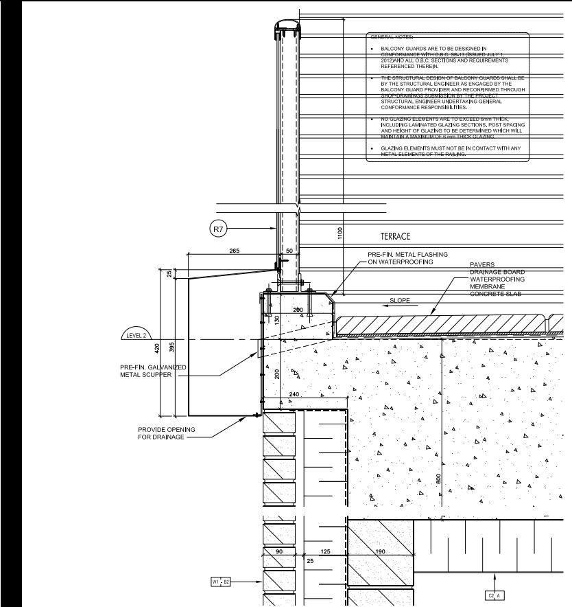
LEVEL TWO SLAB COVER AT EAST RETAIL FACADE (N.T.S.)
