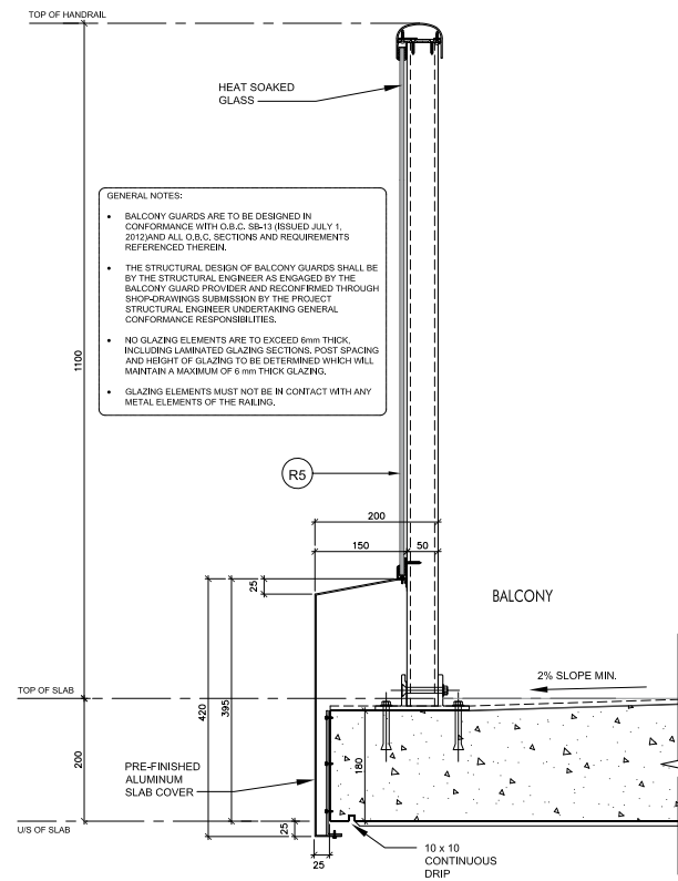
TYPICAL RAILING SECTION AT BALCONY (N.T.S.)
